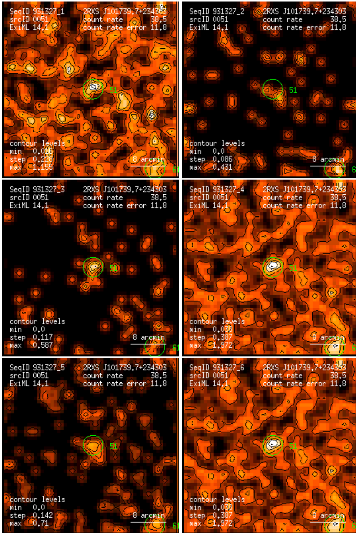
Figure 51: RASS 931327: detection 0051: band rate images, Gaussian filter: (1) PSPC channels 11 – 41, (2) 52 – 90, (3) 91 – 201, (4) 11 – 235, (5) 52 – 201, (6) 11 – 201. Broad band rates in counts/ks. Band rate contour levels in counts/ks/arcmin 2 .
