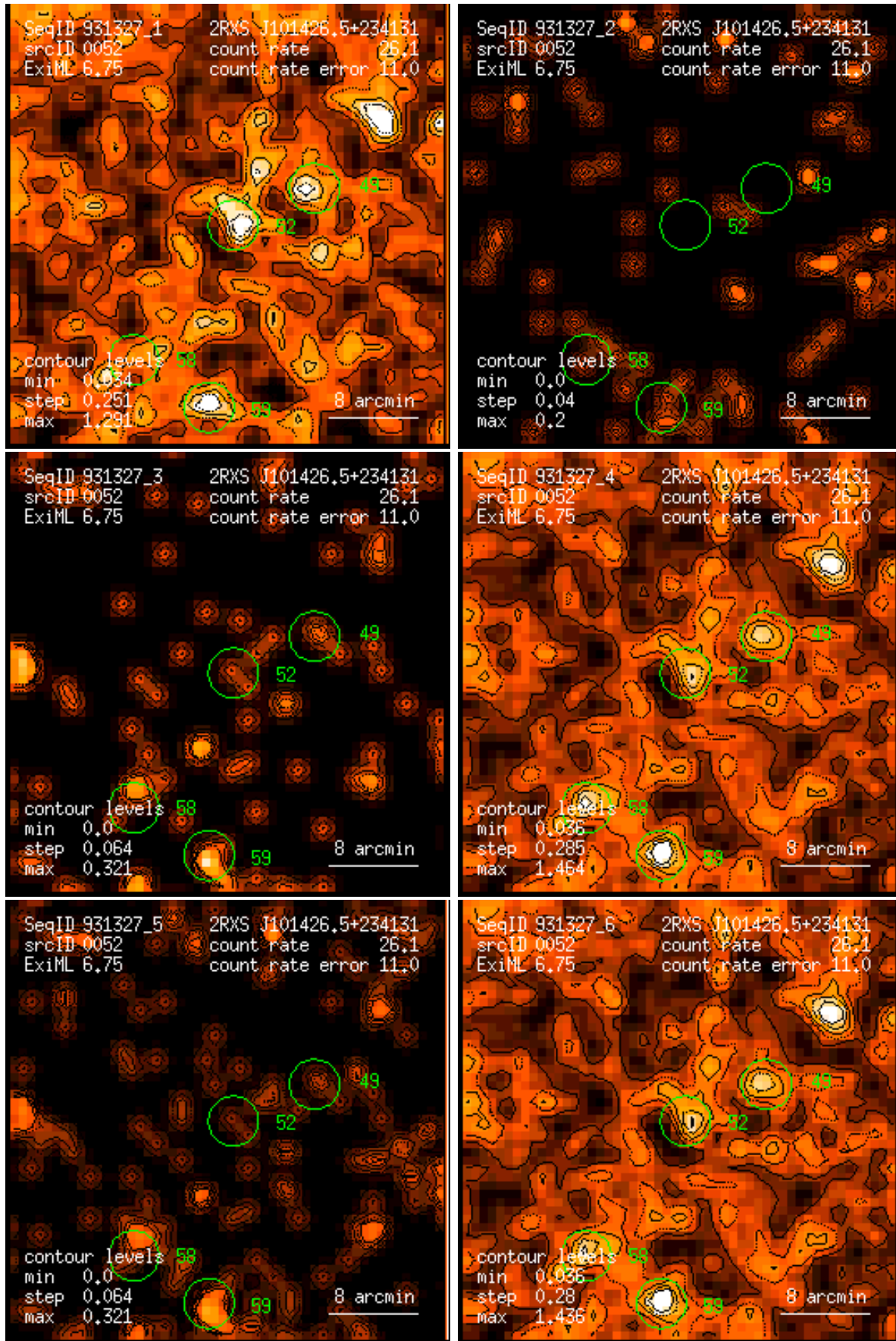
Figure 52: RASS 931327: detection 0052: band rate images, Gaussian filter: (1) PSPC channels 11 – 41, (2) 52 – 90, (3) 91 – 201, (4) 11 – 235, (5) 52 – 201, (6) 11 – 201. Broad band rates in counts/ks. Band rate contour levels in counts/ks/arcmin 2 .
