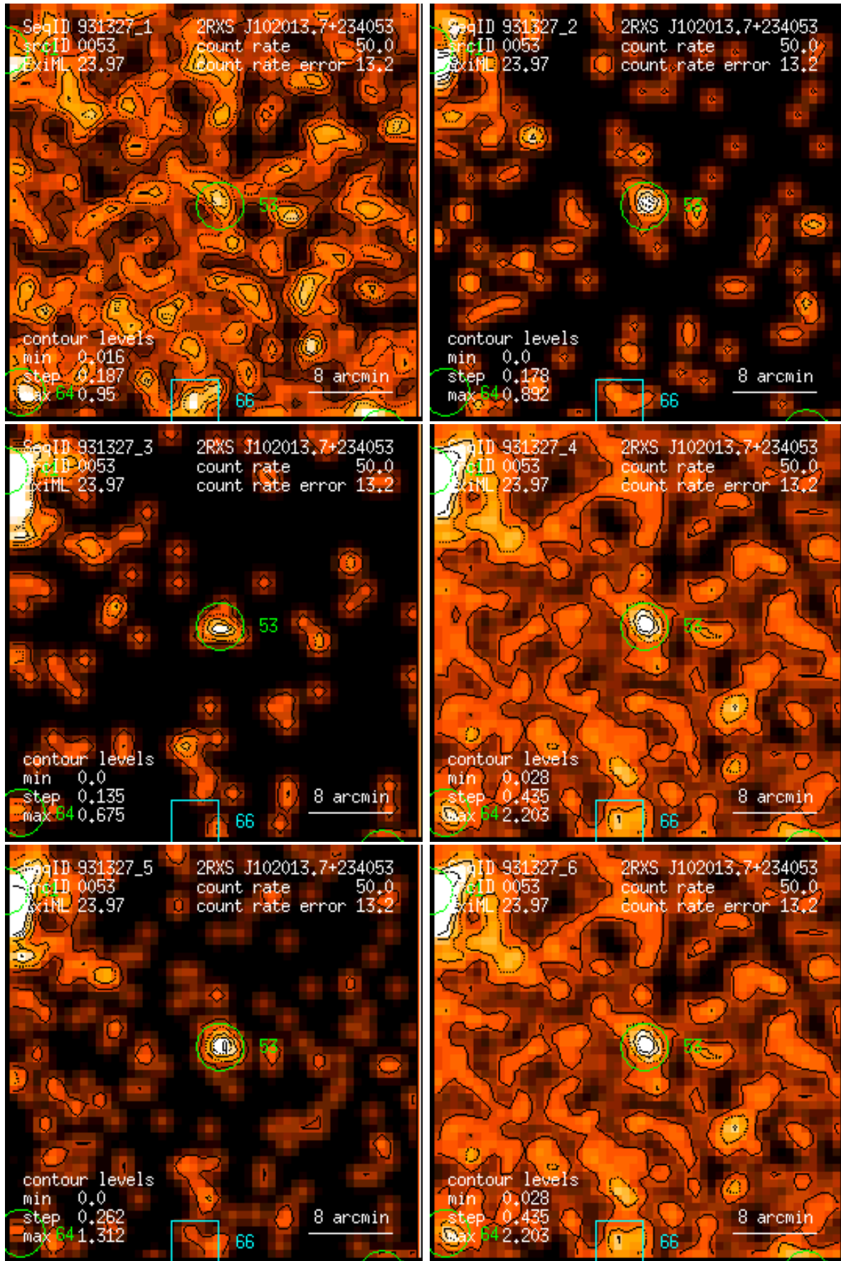
Figure 53: RASS 931327: detection 0053: band rate images, Gaussian filter: (1) PSPC channels 11 – 41, (2) 52 – 90, (3) 91 – 201, (4) 11 – 235, (5) 52 – 201, (6) 11 – 201. Broad band rates in counts/ks. Band rate contour levels in counts/ks/arcmin 2 .
