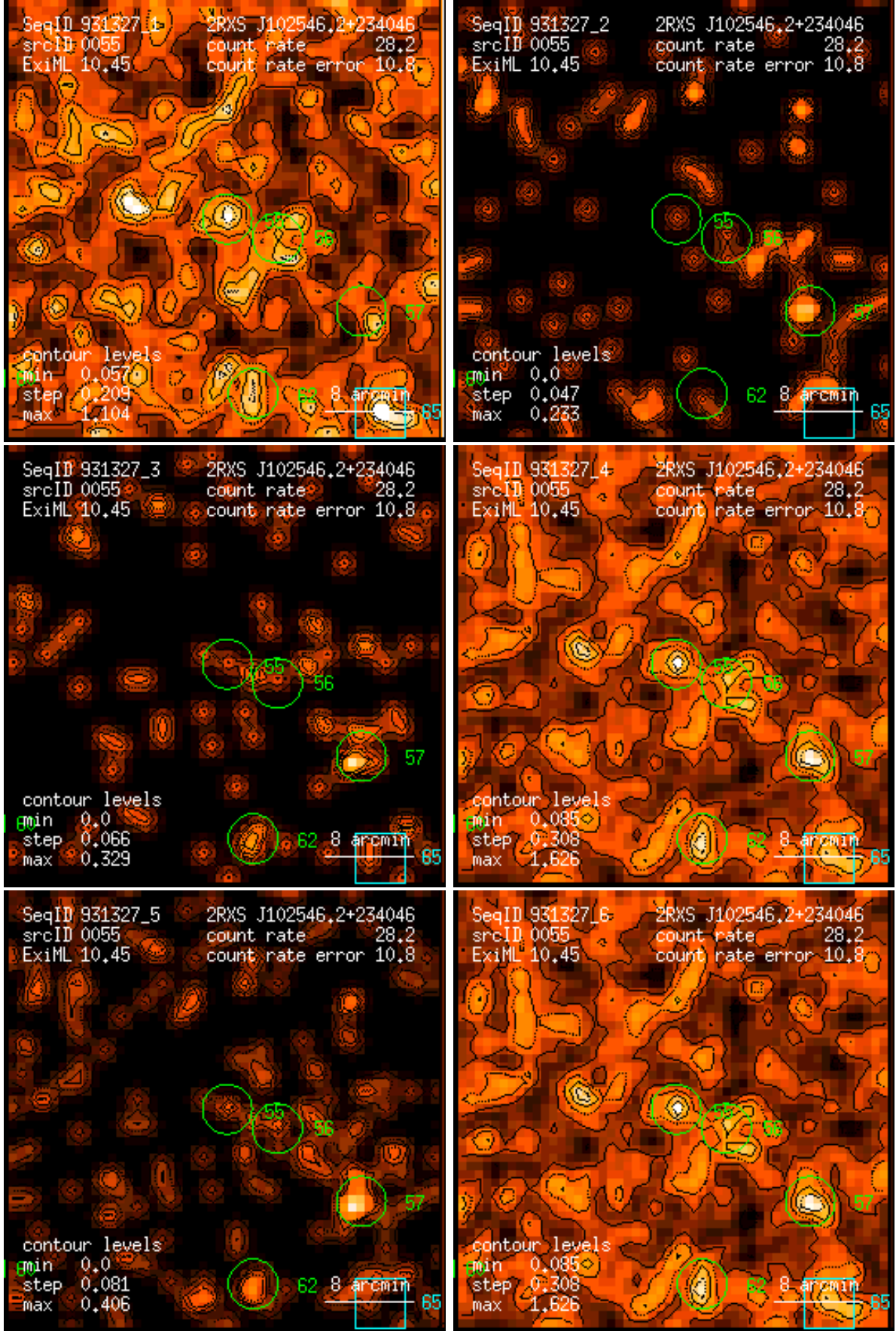
Figure 55: RASS 931327: detection 0055: band rate images, Gaussian filter: (1) PSPC channels 11 – 41, (2) 52 – 90, (3) 91 – 201, (4) 11 – 235, (5) 52 – 201, (6) 11 – 201. Broad band rates in counts/ks. Band rate contour levels in counts/ks/arcmin 2 .
