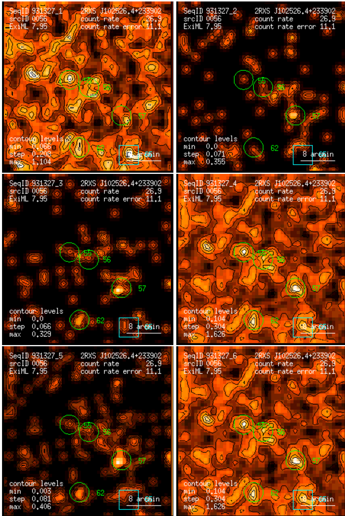
Figure 56: RASS 931327: detection 0056: band rate images, Gaussian filter: (1) PSPC channels 11 – 41, (2) 52 – 90, (3) 91 – 201, (4) 11 – 235, (5) 52 – 201, (6) 11 – 201. Broad band rates in counts/ks. Band rate contour levels in counts/ks/arcmin 2 .
