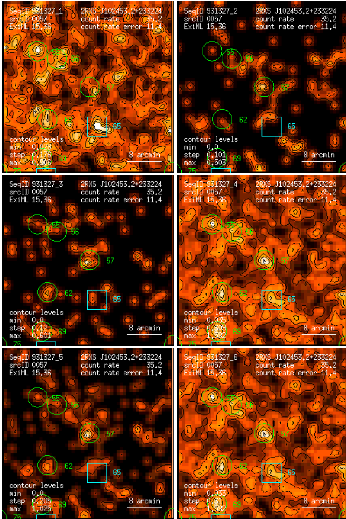
Figure 57: RASS 931327: detection 0057: band rate images, Gaussian filter: (1) PSPC channels 11 – 41, (2) 52 – 90, (3) 91 – 201, (4) 11 – 235, (5) 52 – 201, (6) 11 – 201. Broad band rates in counts/ks. Band rate contour levels in counts/ks/arcmin 2 .
