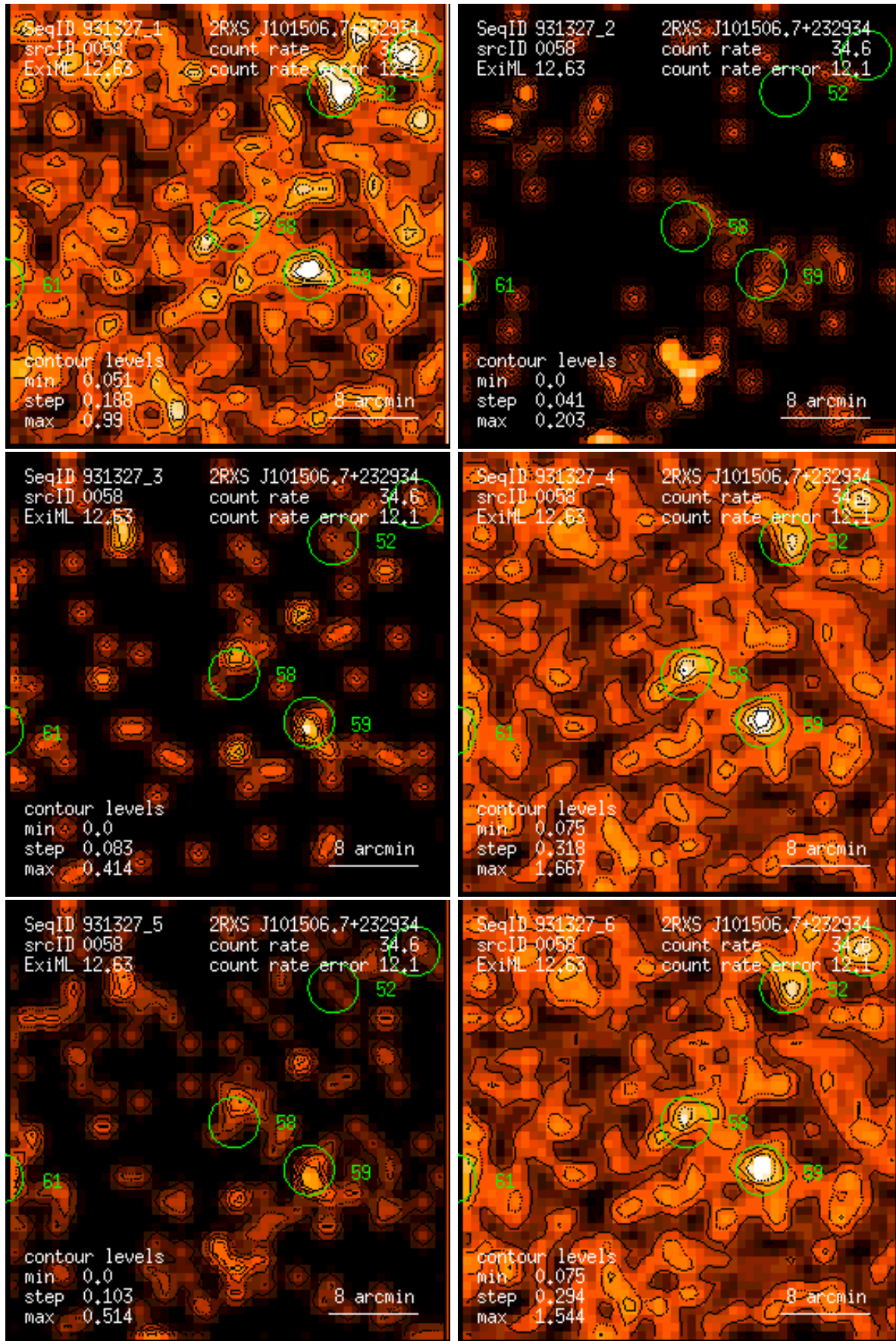
Figure 58: RASS 931327: detection 0058: band rate images, Gaussian filter: (1) PSPC channels 11 – 41, (2) 52 – 90, (3) 91 – 201, (4) 11 – 235, (5) 52 – 201, (6) 11 – 201. Broad band rates in counts/ks. Band rate contour levels in counts/ks/arcmin 2 .
