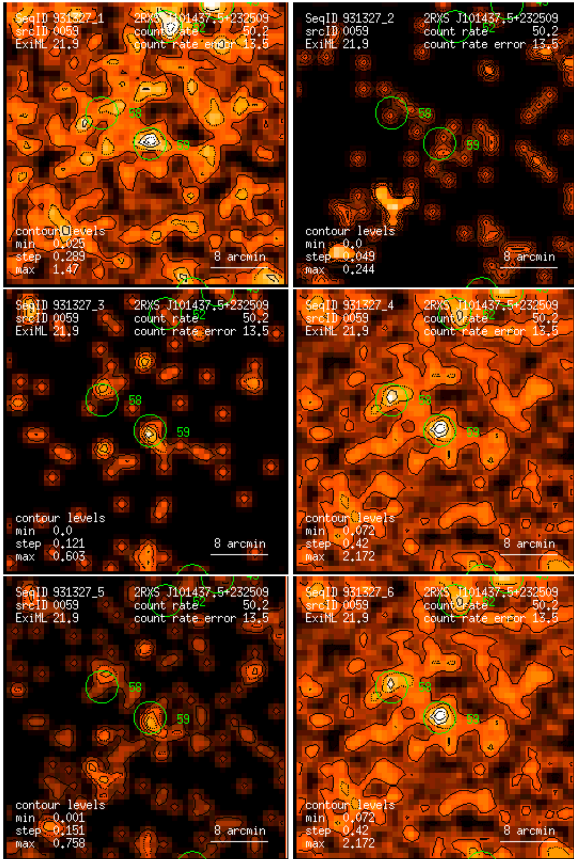
Figure 59: RASS 931327: detection 0059: band rate images, Gaussian filter: (1) PSPC channels 11 – 41, (2) 52 – 90, (3) 91 – 201, (4) 11 – 235, (5) 52 – 201, (6) 11 – 201. Broad band rates in counts/ks. Band rate contour levels in counts/ks/arcmin 2 .
