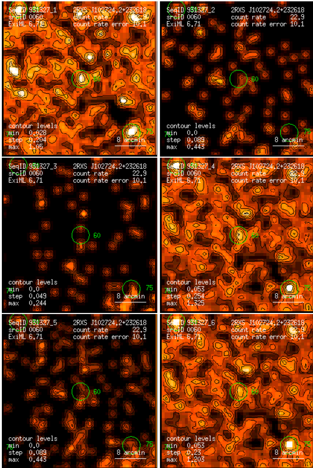
Figure 60: RASS 931327: detection 0060: band rate images, Gaussian filter: (1) PSPC channels 11 – 41, (2) 52 – 90, (3) 91 – 201, (4) 11 – 235, (5) 52 – 201, (6) 11 – 201. Broad band rates in counts/ks. Band rate contour levels in counts/ks/arcmin 2 .
