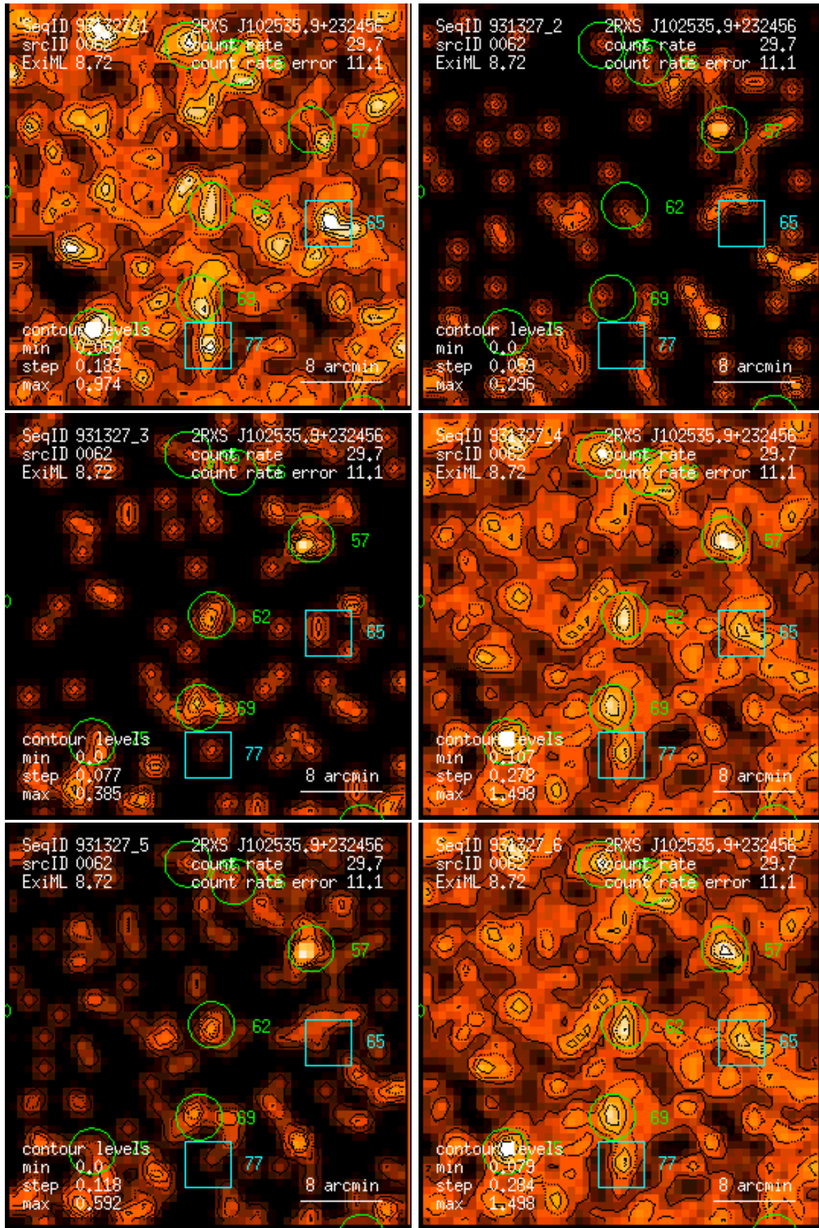
Figure 62: RASS 931327: detection 0062: band rate images, Gaussian filter: (1) PSPC channels 11 – 41, (2) 52 – 90, (3) 91 – 201, (4) 11 – 235, (5) 52 – 201, (6) 11 – 201. Broad band rates in counts/ks. Band rate contour levels in counts/ks/arcmin 2 .
