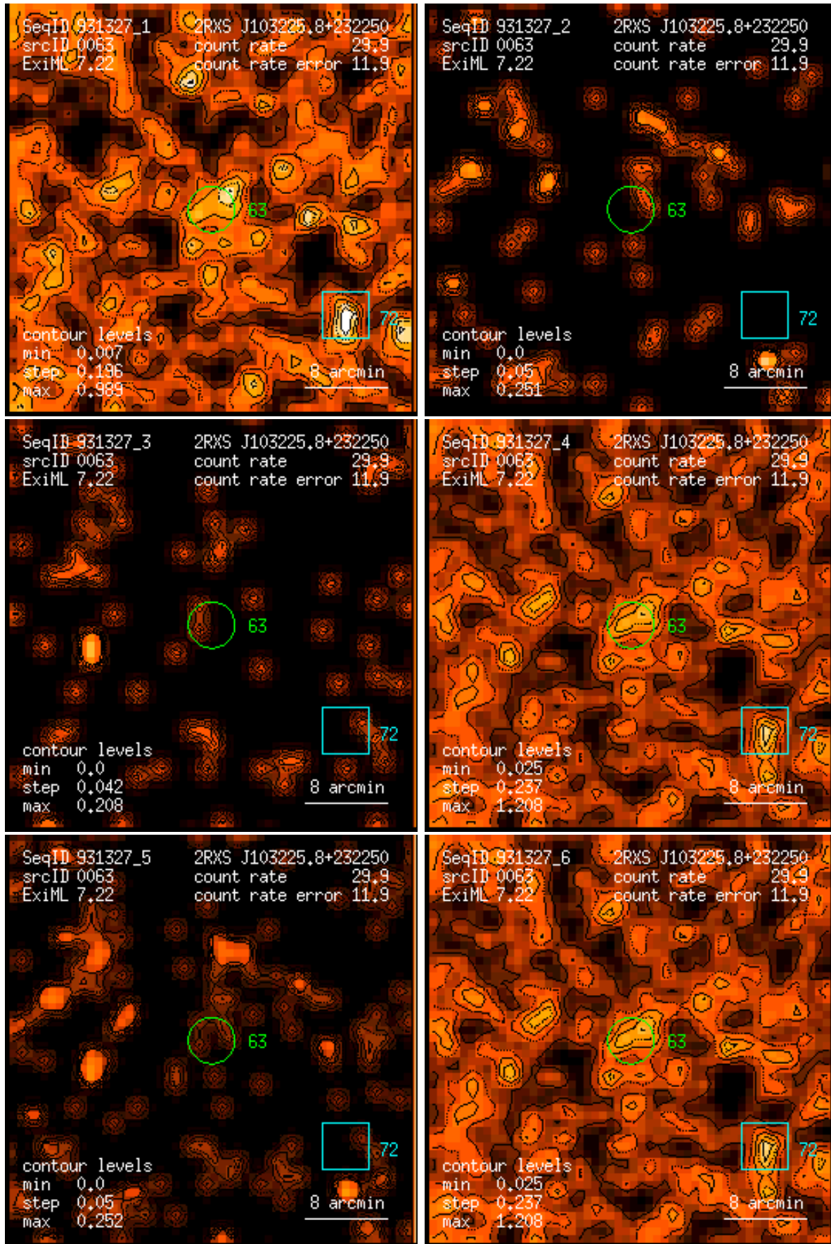
Figure 63: RASS 931327: detection 0063: band rate images, Gaussian filter: (1) PSPC channels 11 – 41, (2) 52 – 90, (3) 91 – 201, (4) 11 – 235, (5) 52 – 201, (6) 11 – 201. Broad band rates in counts/ks. Band rate contour levels in counts/ks/arcmin 2 .
