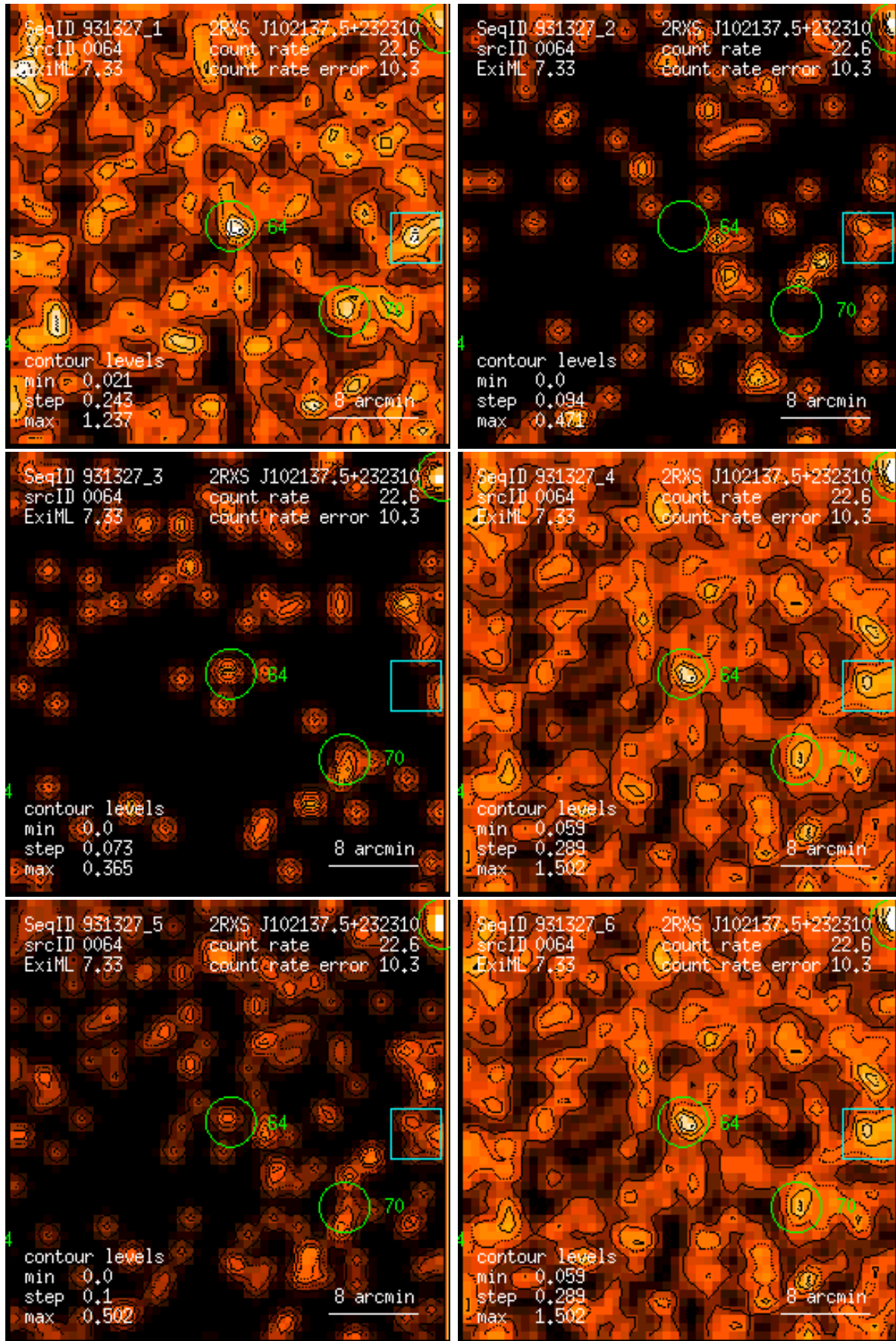
Figure 64: RASS 931327: detection 0064: band rate images, Gaussian filter: (1) PSPC channels 11 – 41, (2) 52 – 90, (3) 91 – 201, (4) 11 – 235, (5) 52 – 201, (6) 11 – 201. Broad band rates in counts/ks. Band rate contour levels in counts/ks/arcmin 2 .
