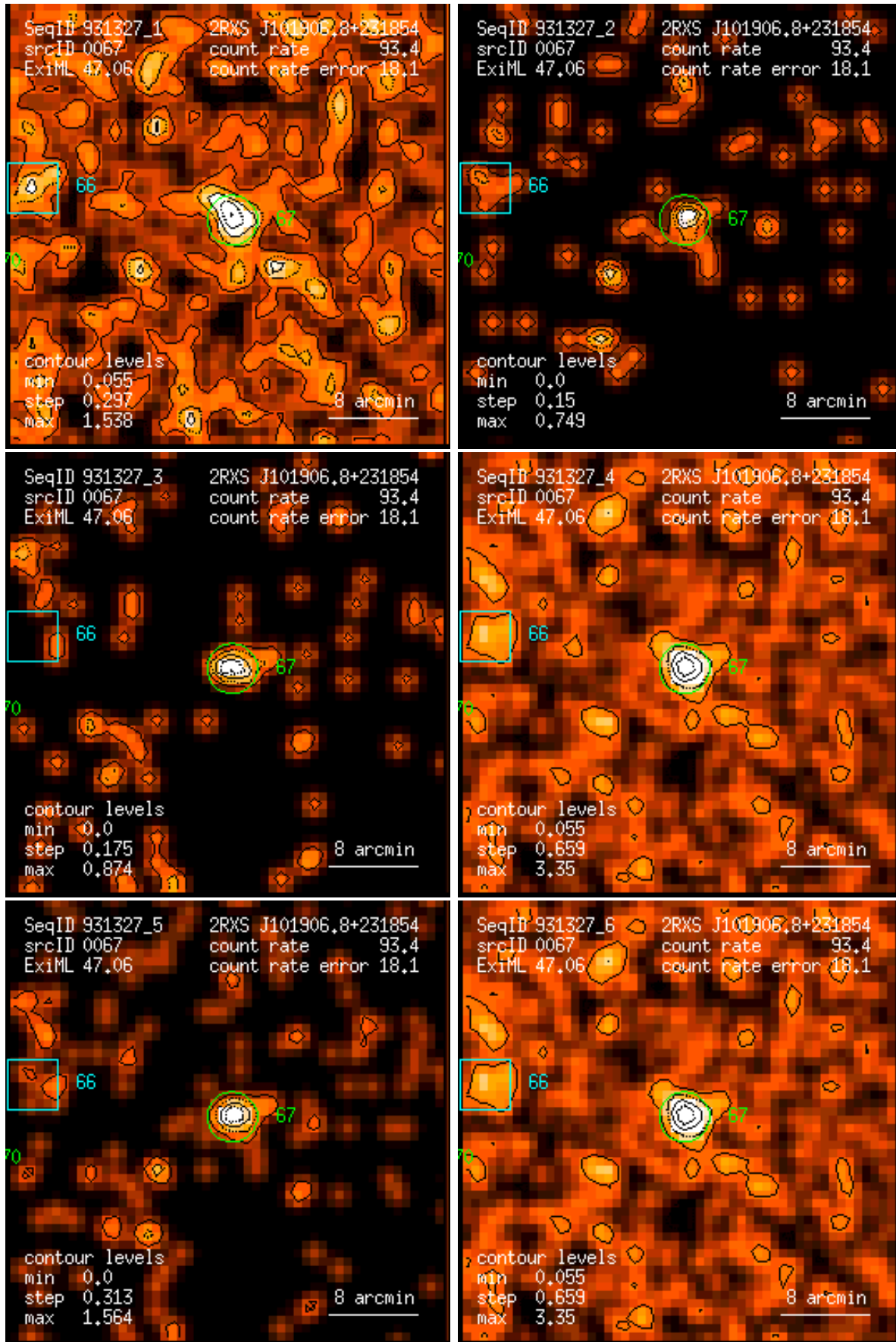
Figure 67: RASS 931327: detection 0067: band rate images, Gaussian filter: (1) PSPC channels 11 – 41, (2) 52 – 90, (3) 91 – 201, (4) 11 – 235, (5) 52 – 201, (6) 11 – 201. Broad band rates in counts/ks. Band rate contour levels in counts/ks/arcmin 2 .
