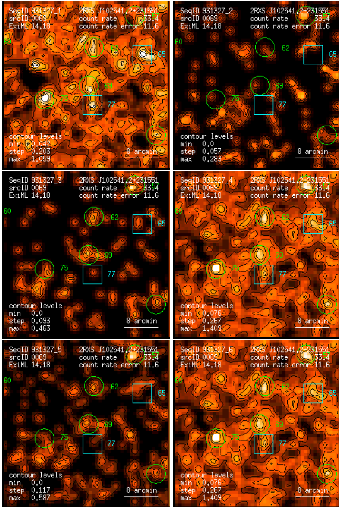
Figure 69: RASS 931327: detection 0069: band rate images, Gaussian filter: (1) PSPC channels 11 – 41, (2) 52 – 90, (3) 91 – 201, (4) 11 – 235, (5) 52 – 201, (6) 11 – 201. Broad band rates in counts/ks. Band rate contour levels in counts/ks/arcmin 2 .
