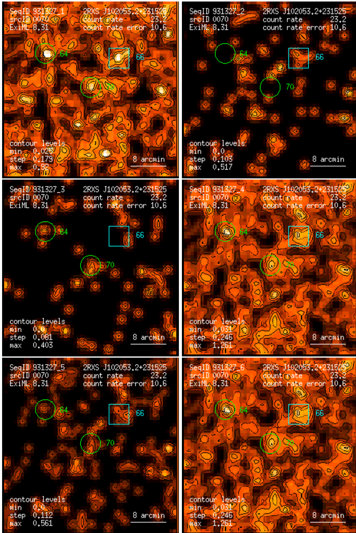
Figure 70: RASS 931327: detection 0070: band rate images, Gaussian filter: (1) PSPC channels 11 – 41, (2) 52 – 90, (3) 91 – 201, (4) 11 – 235, (5) 52 – 201, (6) 11 – 201. Broad band rates in counts/ks. Band rate contour levels in counts/ks/arcmin 2 .
