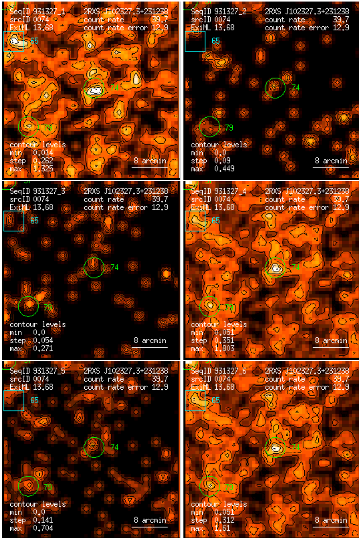
Figure 74: RASS 931327: detection 0074: band rate images, Gaussian filter: (1) PSPC channels 11 – 41, (2) 52 – 90, (3) 91 – 201, (4) 11 – 235, (5) 52 – 201, (6) 11 – 201. Broad band rates in counts/ks. Band rate contour levels in counts/ks/arcmin 2 .
