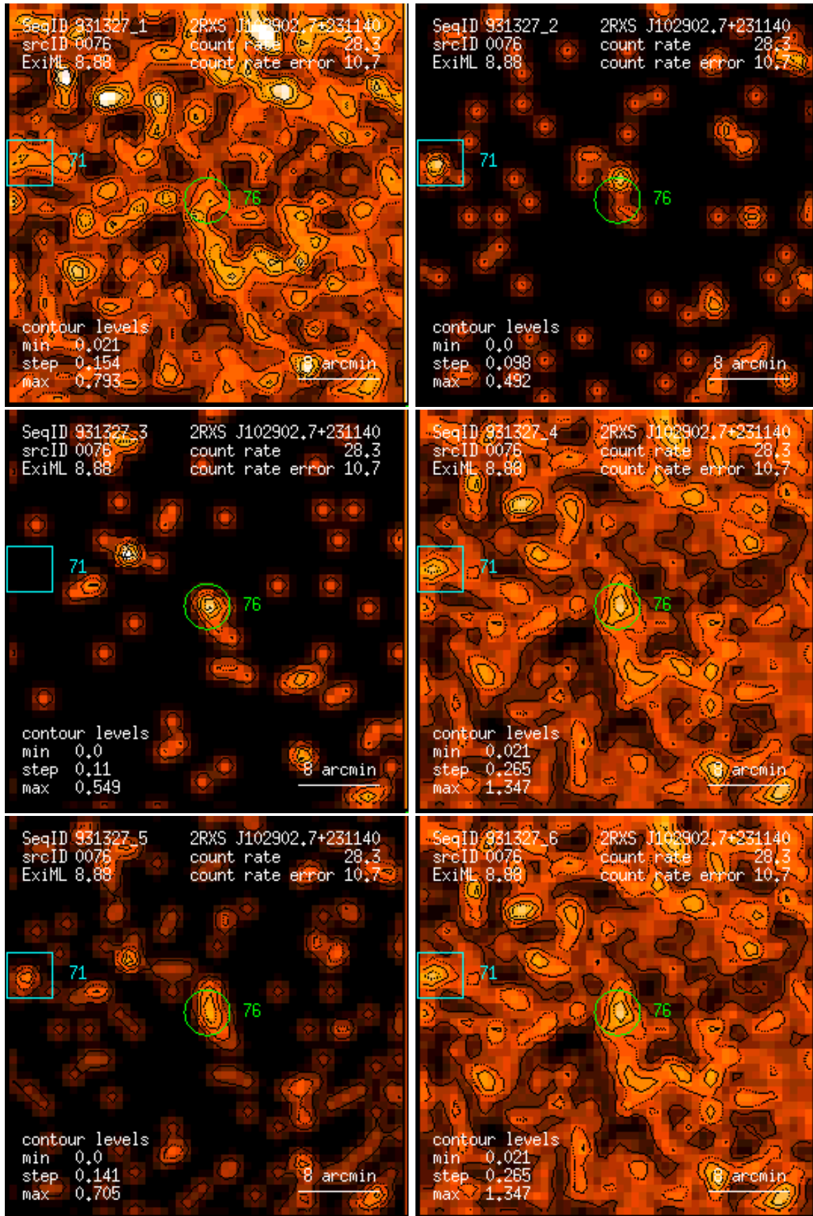
Figure 76: RASS 931327: detection 0076: band rate images, Gaussian filter: (1) PSPC channels 11 – 41, (2) 52 – 90, (3) 91 – 201, (4) 11 – 235, (5) 52 – 201, (6) 11 – 201. Broad band rates in counts/ks. Band rate contour levels in counts/ks/arcmin 2 .
