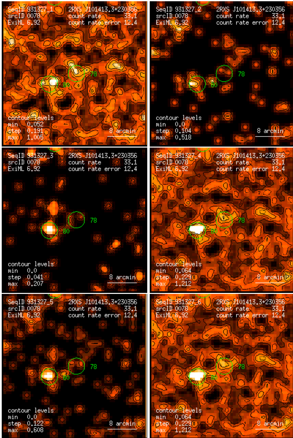
Figure 78: RASS 931327: detection 0078: band rate images, Gaussian filter: (1) PSPC channels 11 – 41, (2) 52 – 90, (3) 91 – 201, (4) 11 – 235, (5) 52 – 201, (6) 11 – 201. Broad band rates in counts/ks. Band rate contour levels in counts/ks/arcmin 2 .
