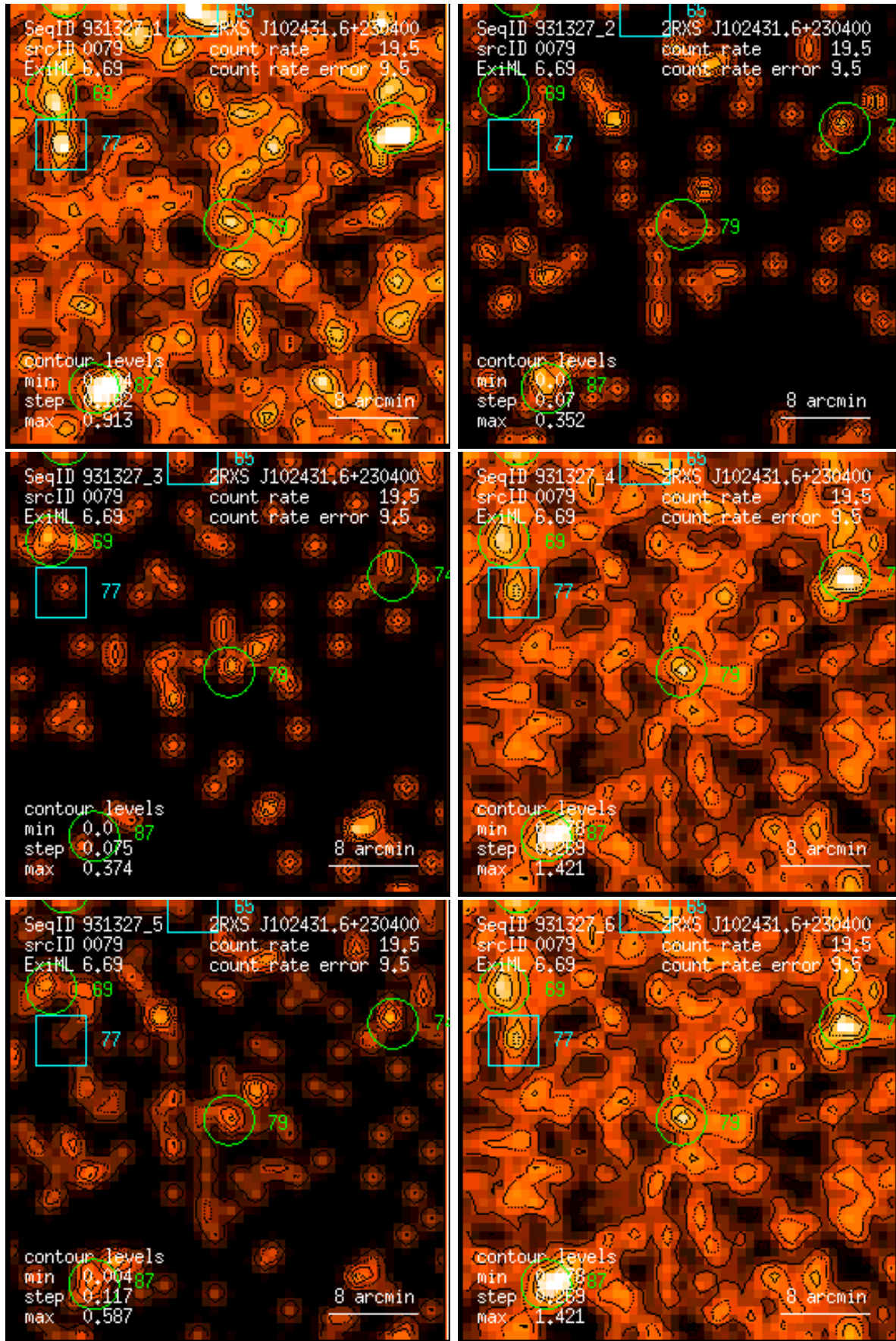
Figure 79: RASS 931327: detection 0079: band rate images, Gaussian filter: (1) PSPC channels 11 – 41, (2) 52 – 90, (3) 91 – 201, (4) 11 – 235, (5) 52 – 201, (6) 11 – 201. Broad band rates in counts/ks. Band rate contour levels in counts/ks/arcmin 2 .
