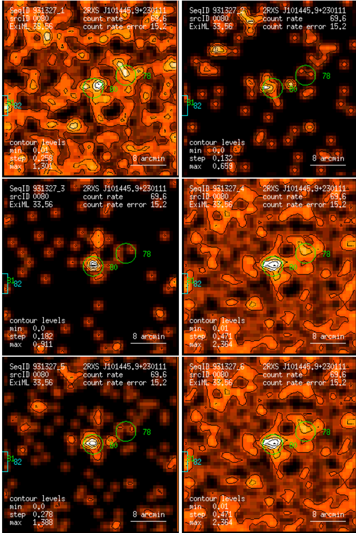
Figure 80: RASS 931327: detection 0080: band rate images, Gaussian filter: (1) PSPC channels 11 – 41, (2) 52 – 90, (3) 91 – 201, (4) 11 – 235, (5) 52 – 201, (6) 11 – 201. Broad band rates in counts/ks. Band rate contour levels in counts/ks/arcmin 2 .
