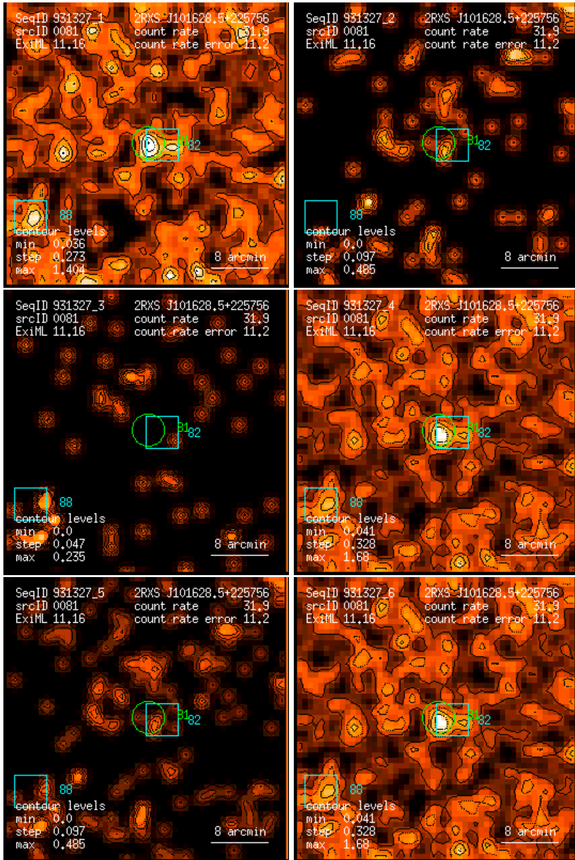
Figure 81: RASS 931327: detection 0081: band rate images, Gaussian filter: (1) PSPC channels 11 – 41, (2) 52 – 90, (3) 91 – 201, (4) 11 – 235, (5) 52 – 201, (6) 11 – 201. Broad band rates in counts/ks. Band rate contour levels in counts/ks/arcmin 2 .
