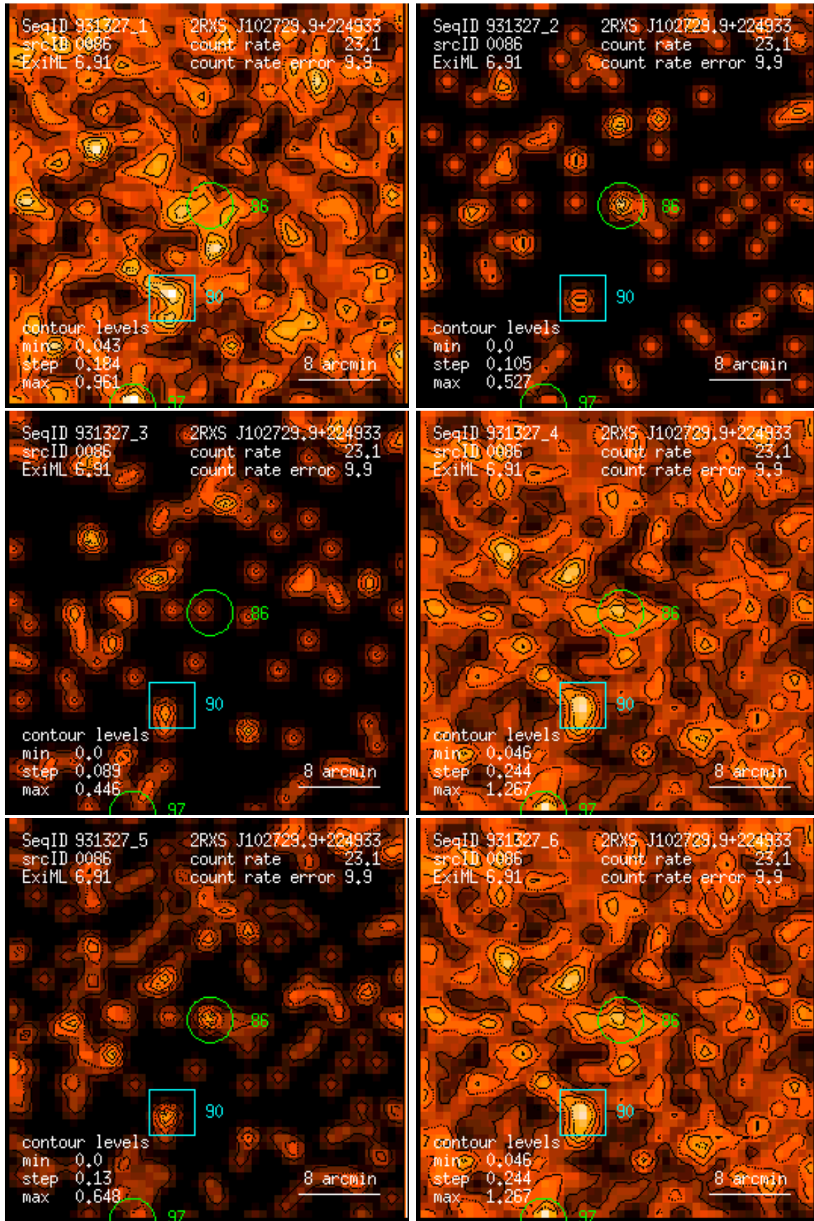
Figure 86: RASS 931327: detection 0086: band rate images, Gaussian filter: (1) PSPC channels 11 – 41, (2) 52 – 90, (3) 91 – 201, (4) 11 – 235, (5) 52 – 201, (6) 11 – 201. Broad band rates in counts/ks. Band rate contour levels in counts/ks/arcmin 2 .
