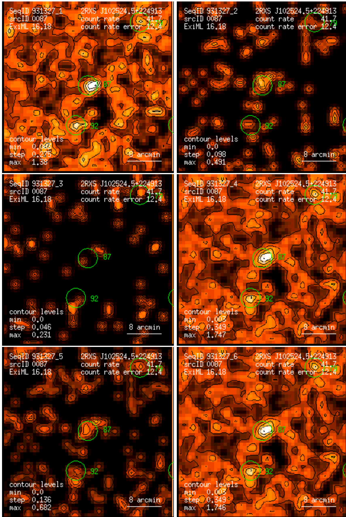
Figure 87: RASS 931327: detection 0087: band rate images, Gaussian filter: (1) PSPC channels 11 – 41, (2) 52 – 90, (3) 91 – 201, (4) 11 – 235, (5) 52 – 201, (6) 11 – 201. Broad band rates in counts/ks. Band rate contour levels in counts/ks/arcmin 2 .
