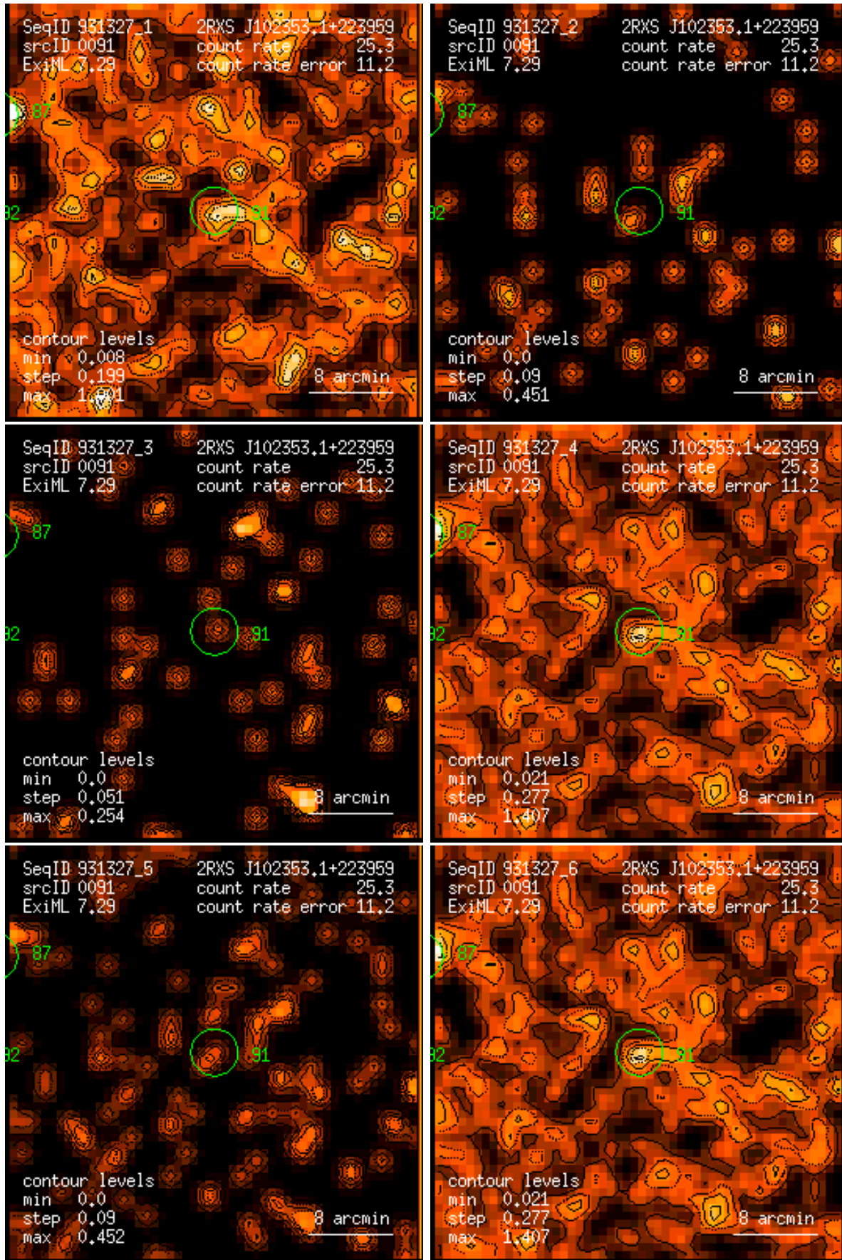
Figure 91: RASS 931327: detection 0091: band rate images, Gaussian filter: (1) PSPC channels 11 – 41, (2) 52 – 90, (3) 91 – 201, (4) 11 – 235, (5) 52 – 201, (6) 11 – 201. Broad band rates in counts/ks. Band rate contour levels in counts/ks/arcmin 2 .
