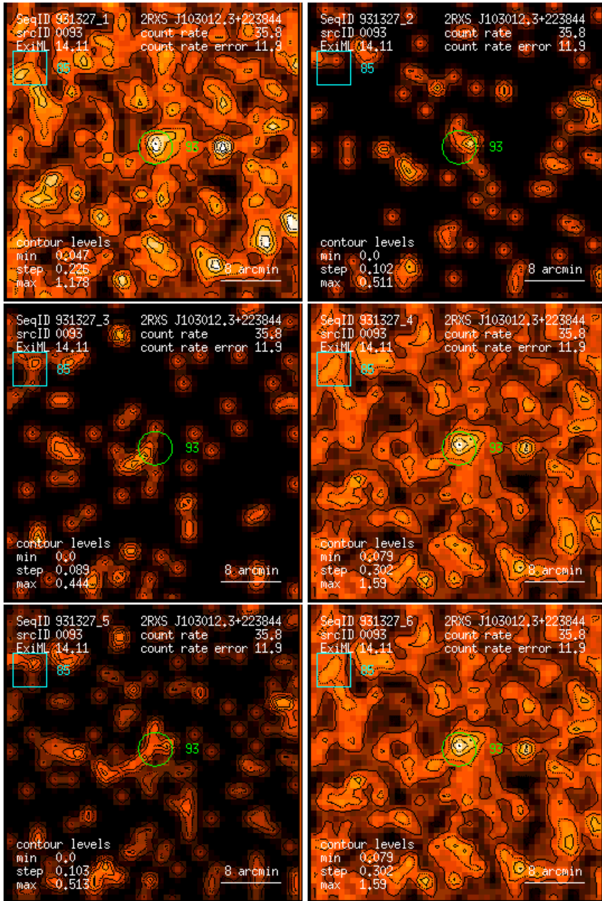
Figure 93: RASS 931327: detection 0093: band rate images, Gaussian filter: (1) PSPC channels 11 – 41, (2) 52 – 90, (3) 91 – 201, (4) 11 – 235, (5) 52 – 201, (6) 11 – 201. Broad band rates in counts/ks. Band rate contour levels in counts/ks/arcmin 2 .
