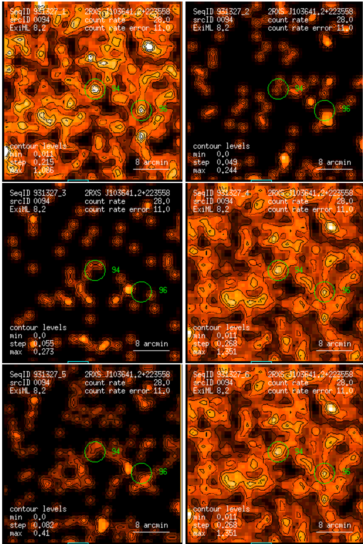
Figure 94: RASS 931327: detection 0094: band rate images, Gaussian filter: (1) PSPC channels 11 – 41, (2) 52 – 90, (3) 91 – 201, (4) 11 – 235, (5) 52 – 201, (6) 11 – 201. Broad band rates in counts/ks. Band rate contour levels in counts/ks/arcmin 2 .
