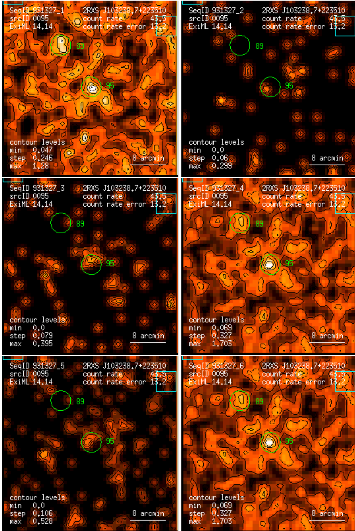
Figure 95: RASS 931327: detection 0095: band rate images, Gaussian filter: (1) PSPC channels 11 – 41, (2) 52 – 90, (3) 91 – 201, (4) 11 – 235, (5) 52 – 201, (6) 11 – 201. Broad band rates in counts/ks. Band rate contour levels in counts/ks/arcmin 2 .
