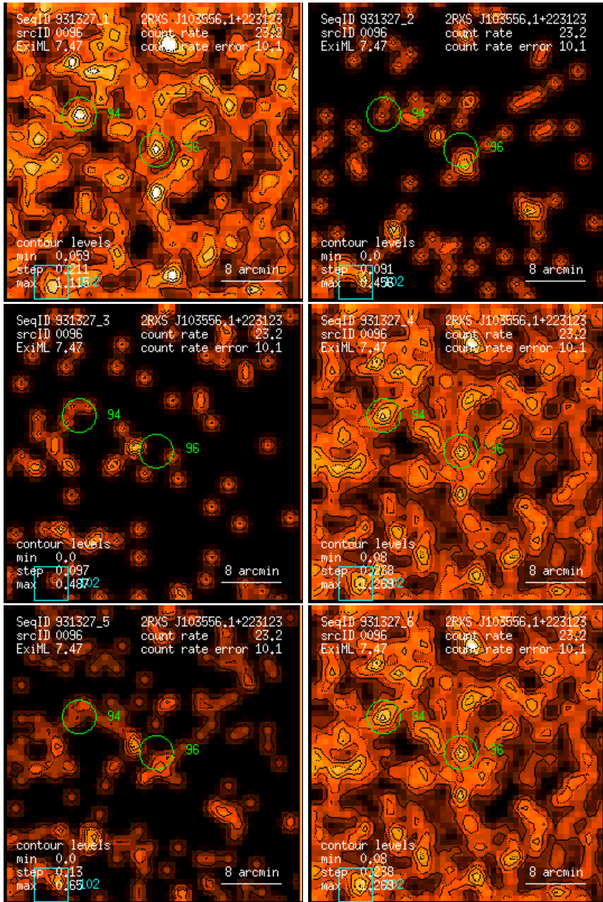
Figure 96: RASS 931327: detection 0096: band rate images, Gaussian filter: (1) PSPC channels 11 – 41, (2) 52 – 90, (3) 91 – 201, (4) 11 – 235, (5) 52 – 201, (6) 11 – 201. Broad band rates in counts/ks. Band rate contour levels in counts/ks/arcmin 2 .
