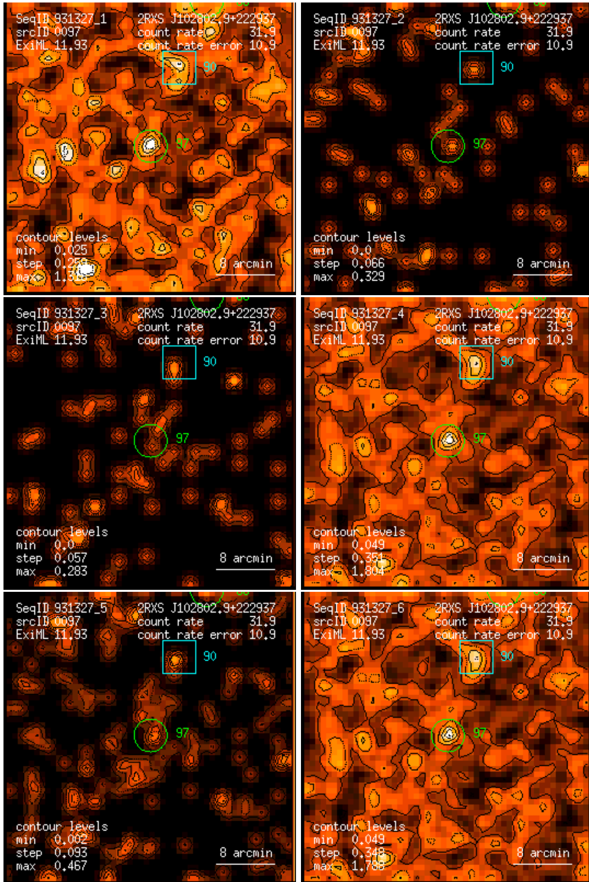
Figure 97: RASS 931327: detection 0097: band rate images, Gaussian filter: (1) PSPC channels 11 – 41, (2) 52 – 90, (3) 91 – 201, (4) 11 – 235, (5) 52 – 201, (6) 11 – 201. Broad band rates in counts/ks. Band rate contour levels in counts/ks/arcmin 2 .
