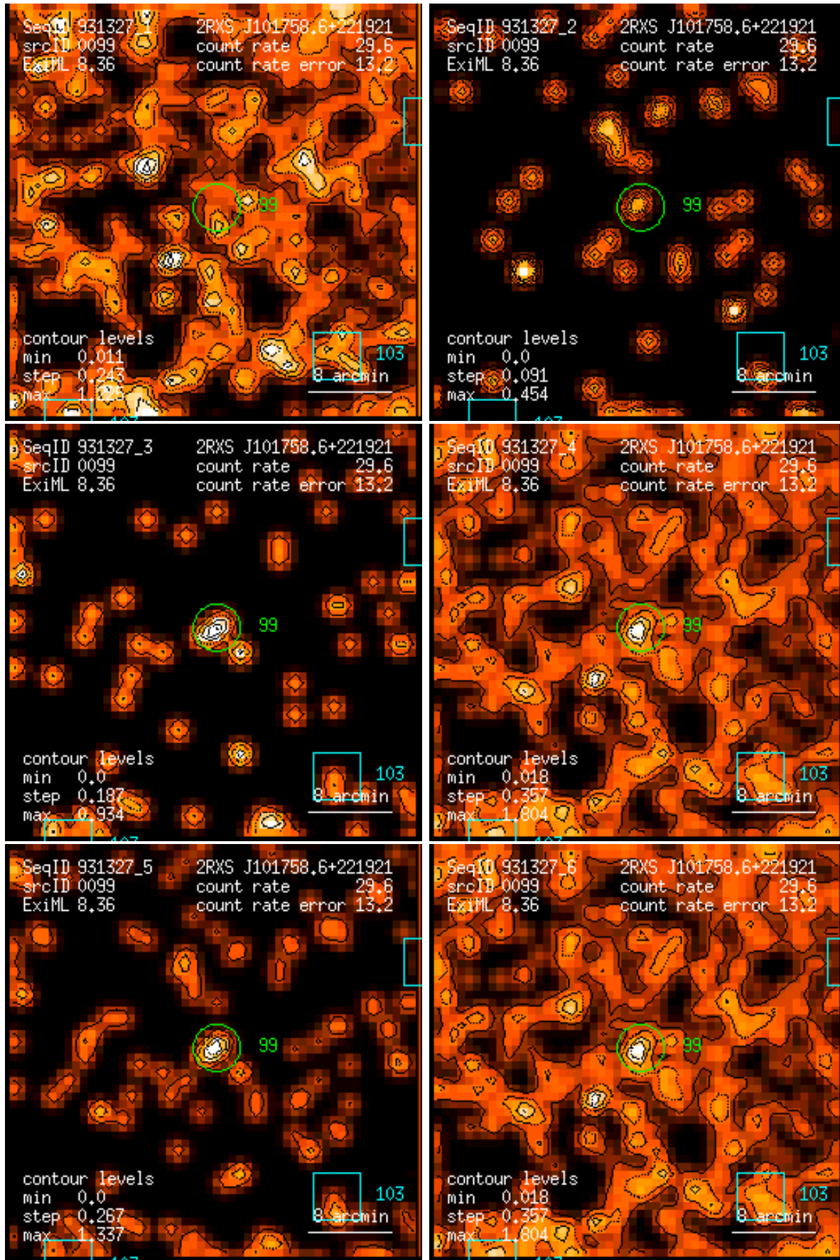
Figure 99: RASS 931327: detection 0099: band rate images, Gaussian filter: (1) PSPC channels 11 – 41, (2) 52 – 90, (3) 91 – 201, (4) 11 – 235, (5) 52 – 201, (6) 11 – 201. Broad band rates in counts/ks. Band rate contour levels in counts/ks/arcmin 2 .
