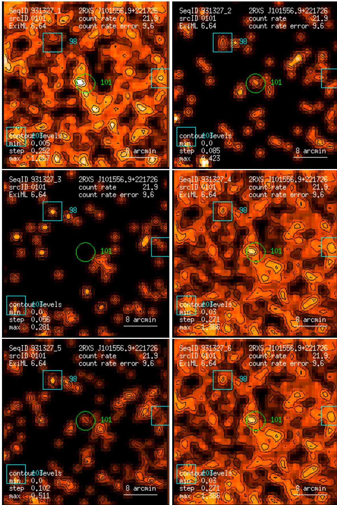
Figure 101: RASS 931327: detection 0101: band rate images, Gaussian filter: (1) PSPC channels 11 – 41, (2) 52 – 90, (3) 91 – 201, (4) 11 – 235, (5) 52 – 201, (6) 11 – 201. Broad band rates in counts/ks. Band rate contour levels in counts/ks/arcmin 2 .
