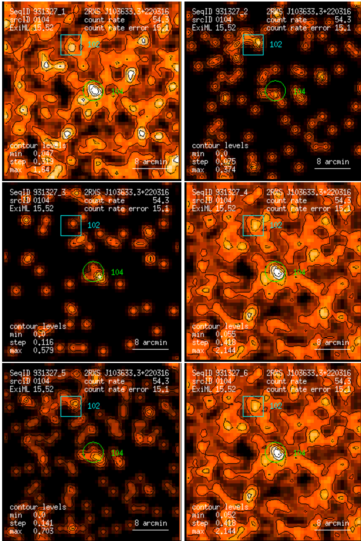
Figure 104: RASS 931327: detection 0104: band rate images, Gaussian filter: (1) PSPC channels 11 – 41, (2) 52 – 90, (3) 91 – 201, (4) 11 – 235, (5) 52 – 201, (6) 11 – 201. Broad band rates in counts/ks. Band rate contour levels in counts/ks/arcmin 2 .
