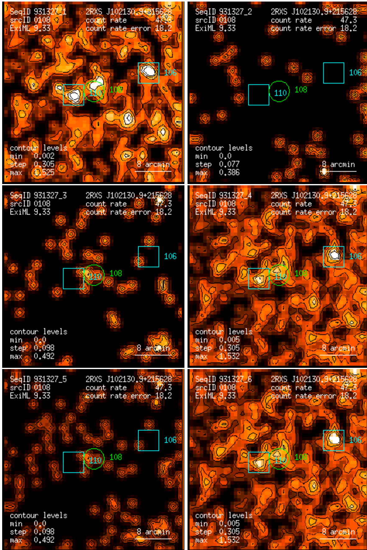
Figure 108: RASS 931327: detection 0108: band rate images, Gaussian filter: (1) PSPC channels 11 – 41, (2) 52 – 90, (3) 91 – 201, (4) 11 – 235, (5) 52 – 201, (6) 11 – 201. Broad band rates in counts/ks. Band rate contour levels in counts/ks/arcmin 2 .
