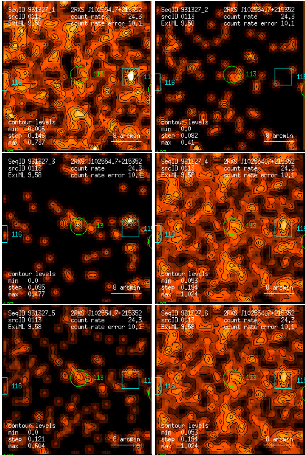
Figure 113: RASS 931327: detection 0113: band rate images, Gaussian filter: (1) PSPC channels 11 – 41, (2) 52 – 90, (3) 91 – 201, (4) 11 – 235, (5) 52 – 201, (6) 11 – 201. Broad band rates in counts/ks. Band rate contour levels in counts/ks/arcmin 2 .
