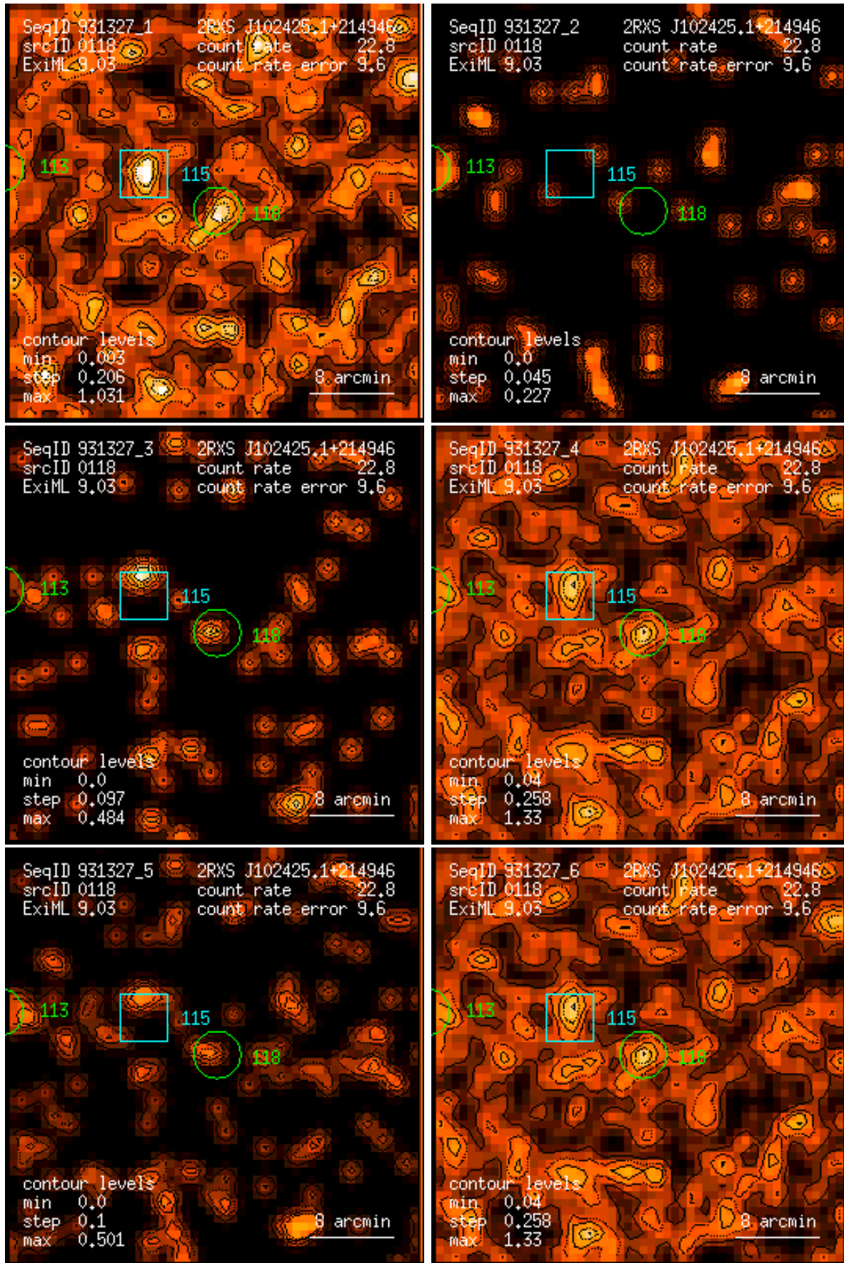
Figure 118: RASS 931327: detection 0118: band rate images, Gaussian filter: (1) PSPC channels 11 – 41, (2) 52 – 90, (3) 91 – 201, (4) 11 – 235, (5) 52 – 201, (6) 11 – 201. Broad band rates in counts/ks. Band rate contour levels in counts/ks/arcmin 2 .
