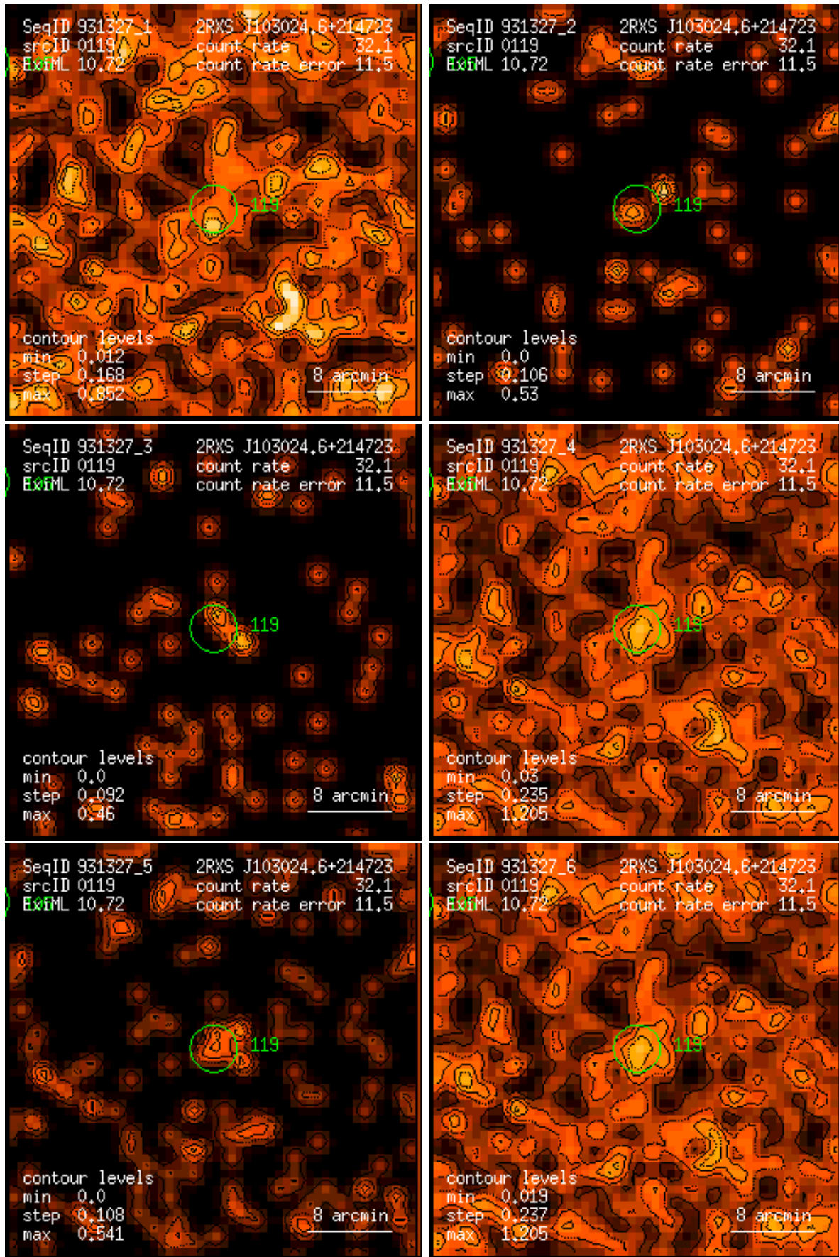
Figure 119: RASS 931327: detection 0119: band rate images, Gaussian filter: (1) PSPC channels 11 – 41, (2) 52 – 90, (3) 91 – 201, (4) 11 – 235, (5) 52 – 201, (6) 11 – 201. Broad band rates in counts/ks. Band rate contour levels in counts/ks/arcmin 2 .
