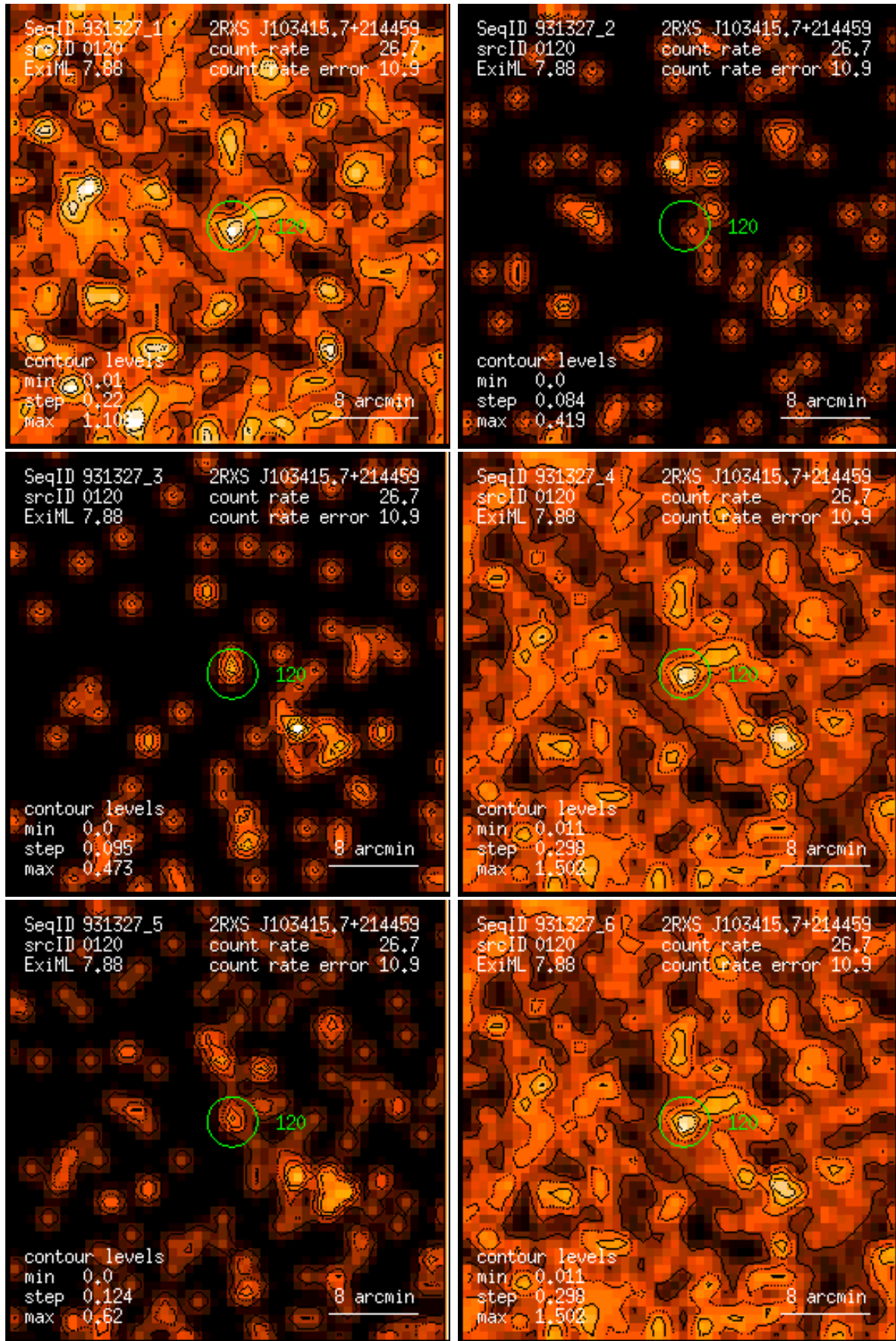
Figure 120: RASS 931327: detection 0120: band rate images, Gaussian filter: (1) PSPC channels 11 – 41, (2) 52 – 90, (3) 91 – 201, (4) 11 – 235, (5) 52 – 201, (6) 11 – 201. Broad band rates in counts/ks. Band rate contour levels in counts/ks/arcmin 2 .
