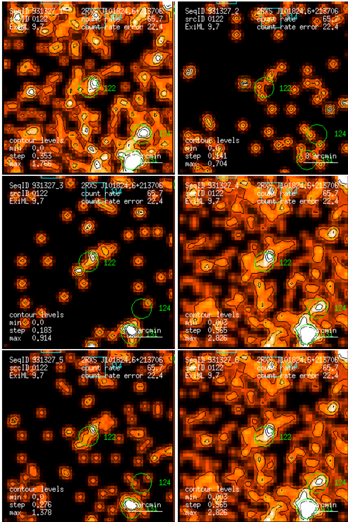
Figure 122: RASS 931327: detection 0122: band rate images, Gaussian filter: (1) PSPC channels 11 – 41, (2) 52 – 90, (3) 91 – 201, (4) 11 – 235, (5) 52 – 201, (6) 11 – 201. Broad band rates in counts/ks. Band rate contour levels in counts/ks/arcmin 2 .
