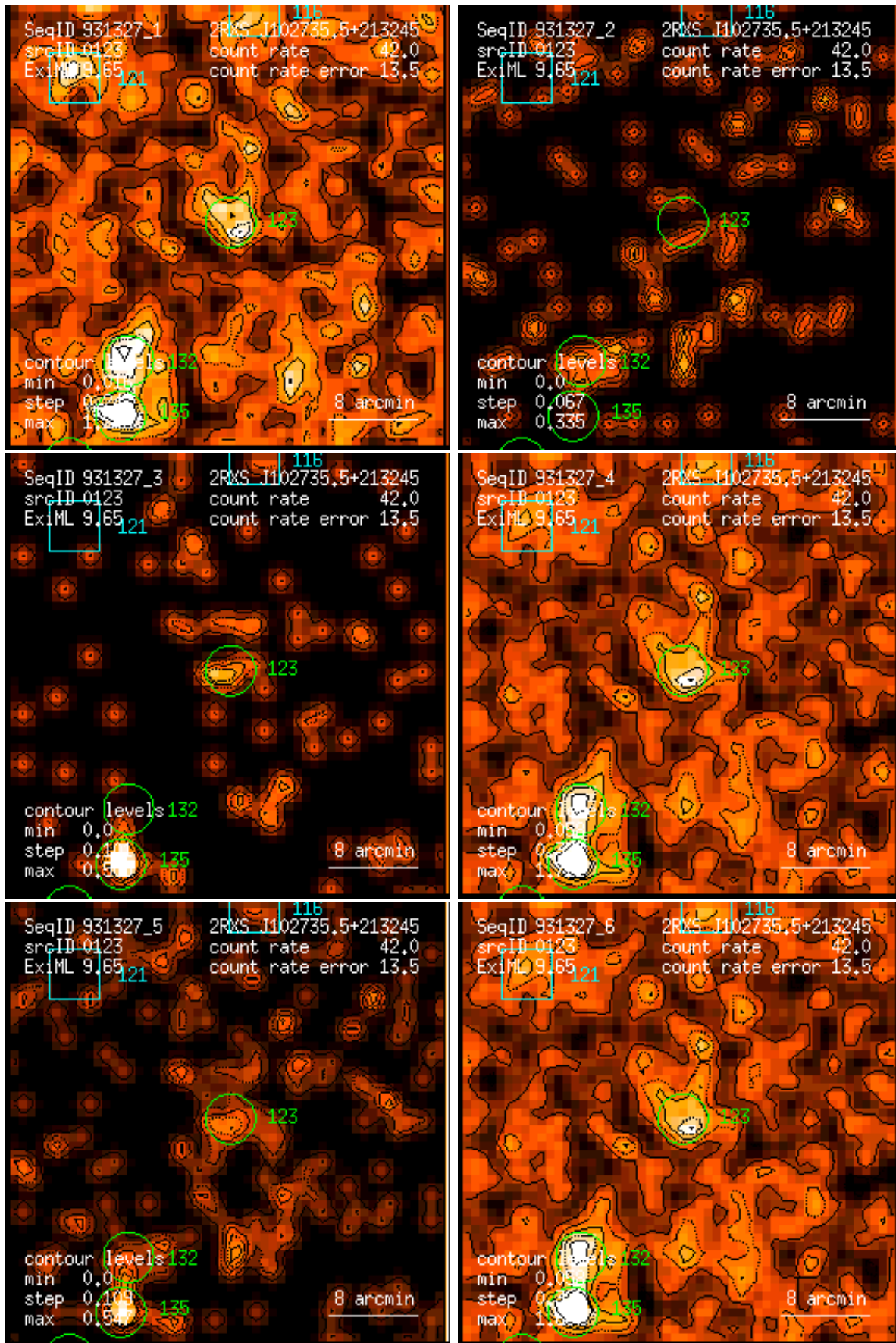
Figure 123: RASS 931327: detection 0123: band rate images, Gaussian filter: (1) PSPC channels 11 – 41, (2) 52 – 90, (3) 91 – 201, (4) 11 – 235, (5) 52 – 201, (6) 11 – 201. Broad band rates in counts/ks. Band rate contour levels in counts/ks/arcmin 2 .
