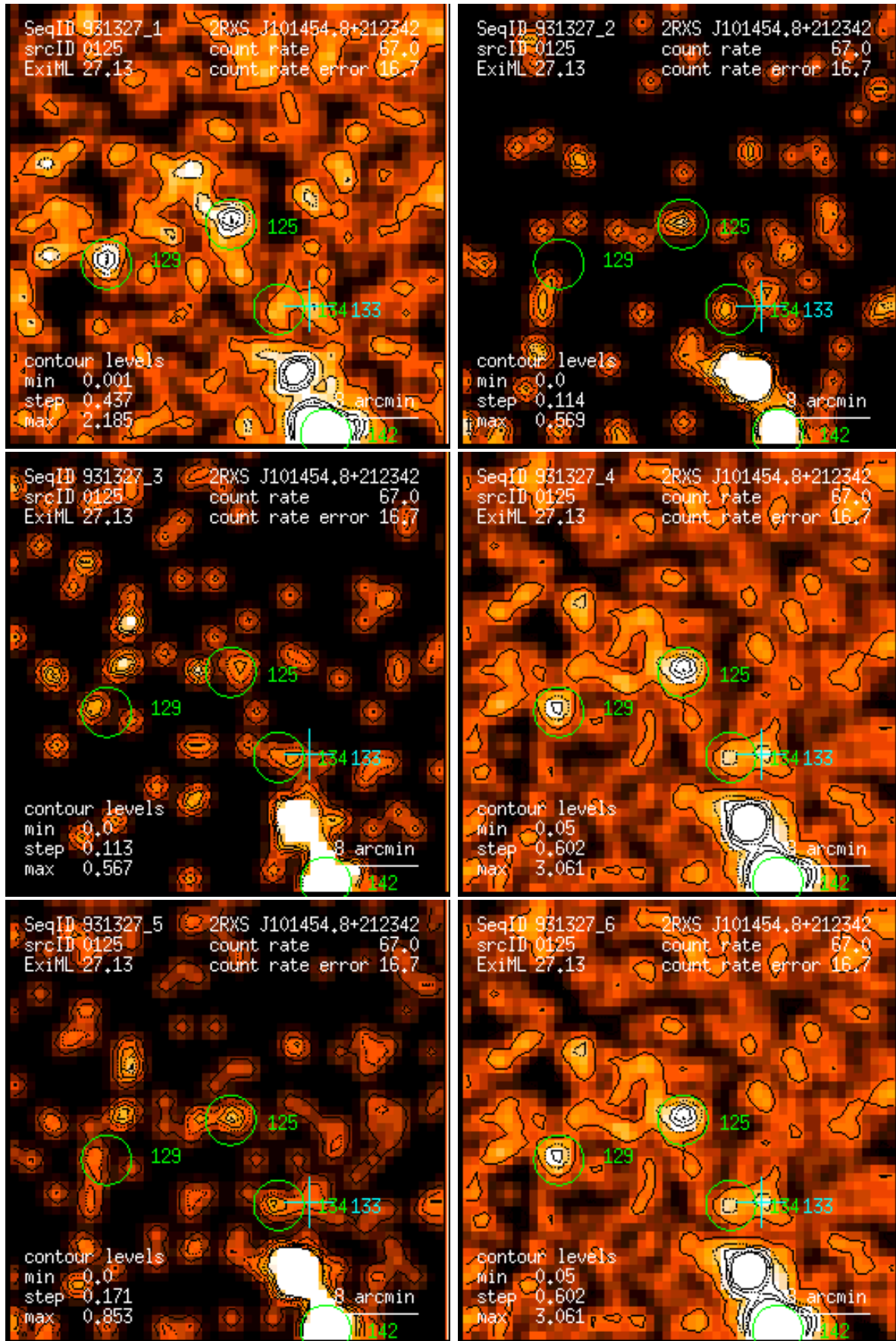
Figure 125: RASS 931327: detection 0125: band rate images, Gaussian filter: (1) PSPC channels 11 – 41, (2) 52 – 90, (3) 91 – 201, (4) 11 – 235, (5) 52 – 201, (6) 11 – 201. Broad band rates in counts/ks. Band rate contour levels in counts/ks/arcmin 2 .
