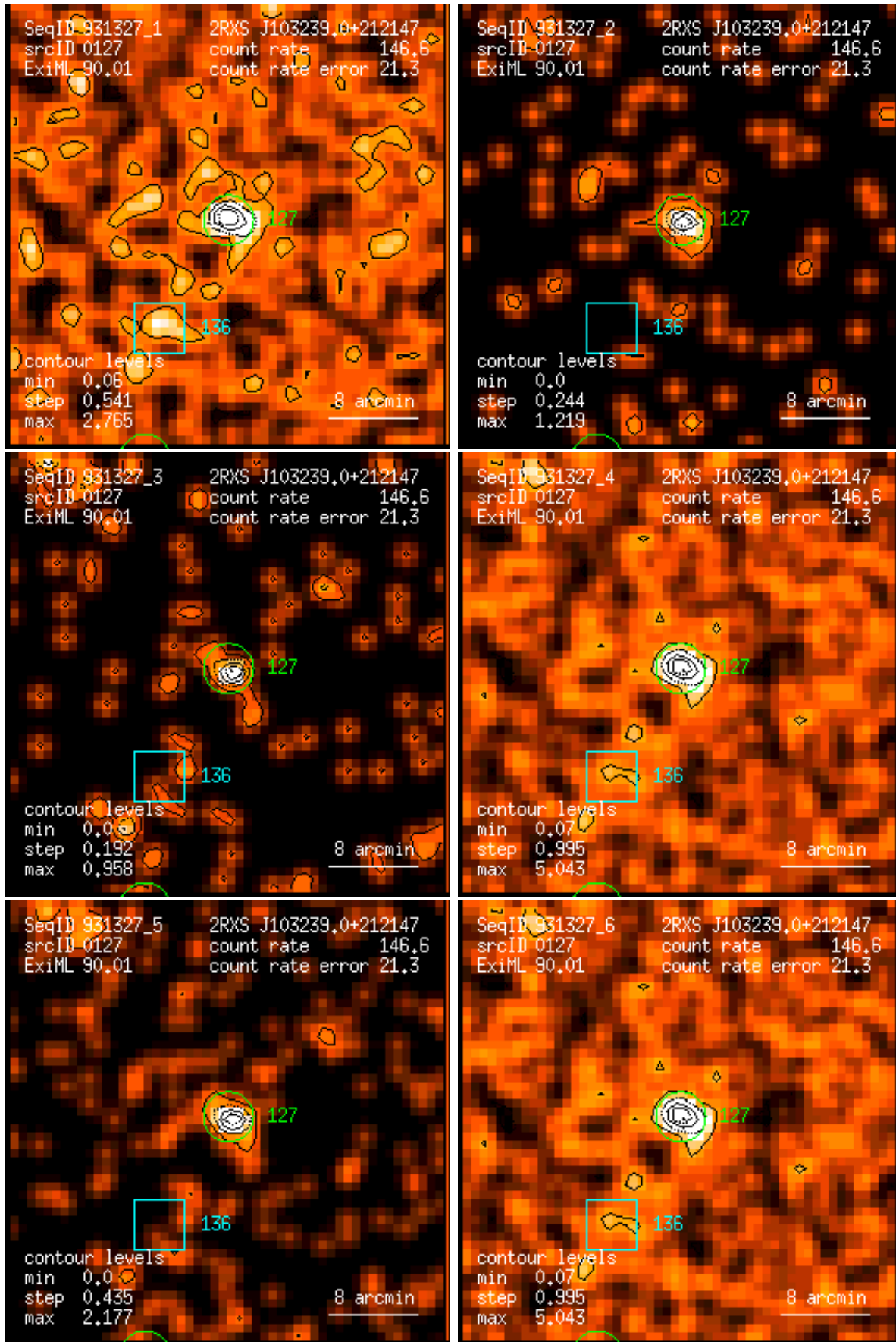
Figure 127: RASS 931327: detection 0127: band rate images, Gaussian filter: (1) PSPC channels 11 – 41, (2) 52 – 90, (3) 91 – 201, (4) 11 – 235, (5) 52 – 201, (6) 11 – 201. Broad band rates in counts/ks. Band rate contour levels in counts/ks/arcmin 2 .
