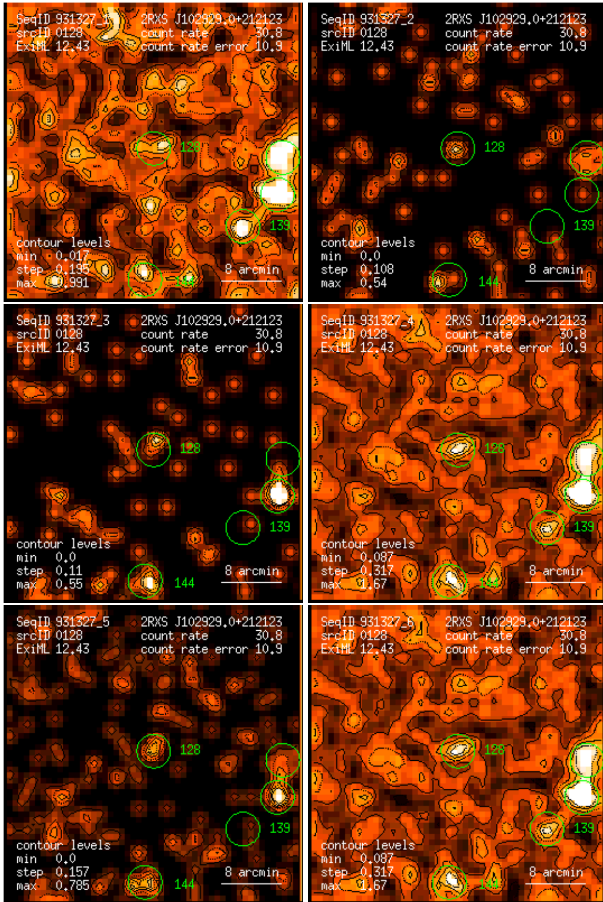
Figure 128: RASS 931327: detection 0128: band rate images, Gaussian filter: (1) PSPC channels 11 – 41, (2) 52 – 90, (3) 91 – 201, (4) 11 – 235, (5) 52 – 201, (6) 11 – 201. Broad band rates in counts/ks. Band rate contour levels in counts/ks/arcmin 2 .
