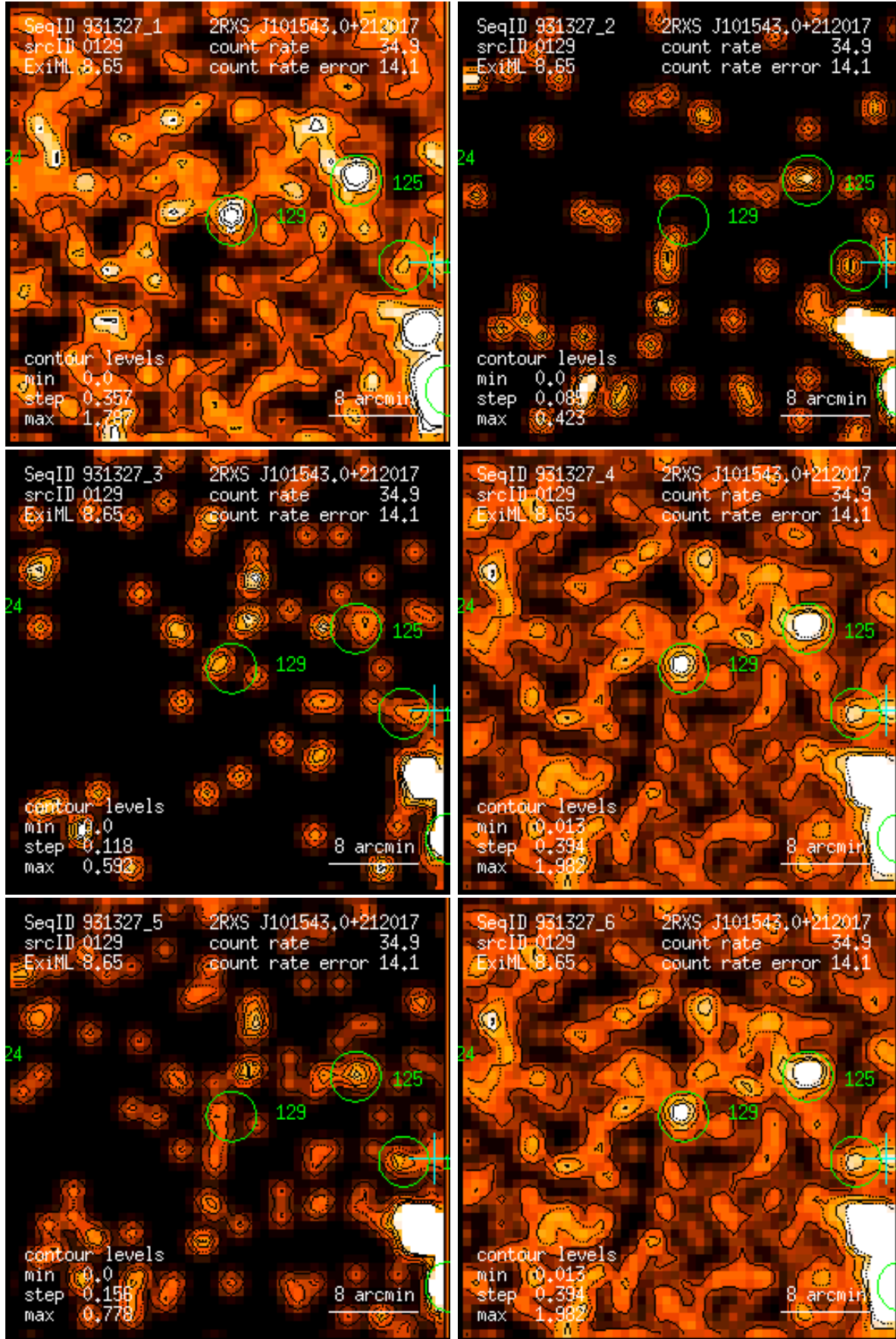
Figure 129: RASS 931327: detection 0129: band rate images, Gaussian filter: (1) PSPC channels 11 – 41, (2) 52 – 90, (3) 91 – 201, (4) 11 – 235, (5) 52 – 201, (6) 11 – 201. Broad band rates in counts/ks. Band rate contour levels in counts/ks/arcmin 2 .
