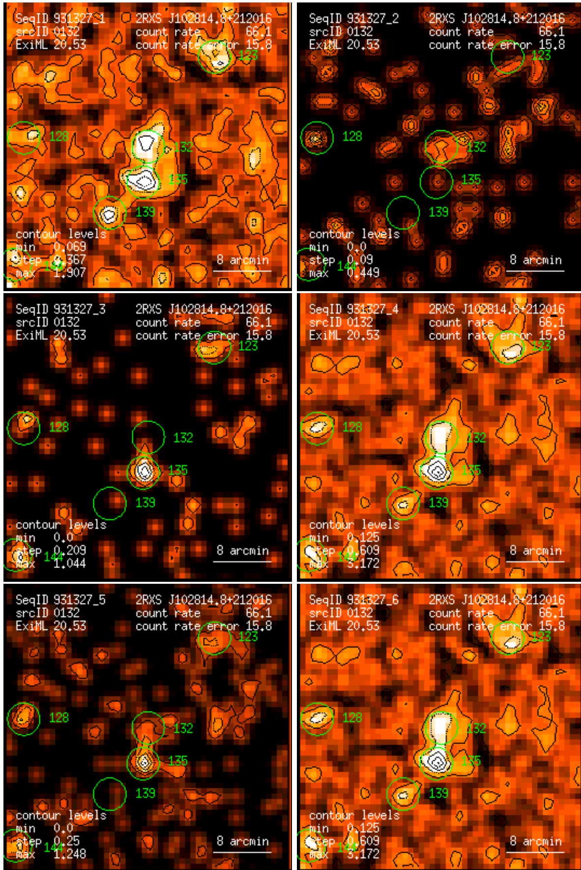
Figure 132: RASS 931327: detection 0132: band rate images, Gaussian filter: (1) PSPC channels 11 – 41, (2) 52 – 90, (3) 91 – 201, (4) 11 – 235, (5) 52 – 201, (6) 11 – 201. Broad band rates in counts/ks. Band rate contour levels in counts/ks/arcmin 2 .
