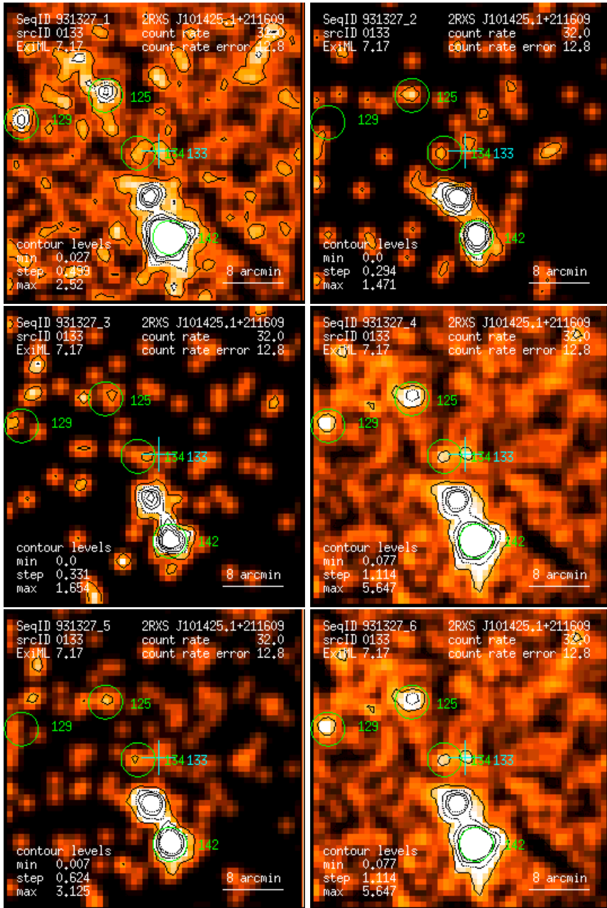
Figure 133: RASS 931327: detection 0133: band rate images, Gaussian filter: (1) PSPC channels 11 – 41, (2) 52 – 90, (3) 91 – 201, (4) 11 – 235, (5) 52 – 201, (6) 11 – 201. Broad band rates in counts/ks. Band rate contour levels in counts/ks/arcmin 2 .
