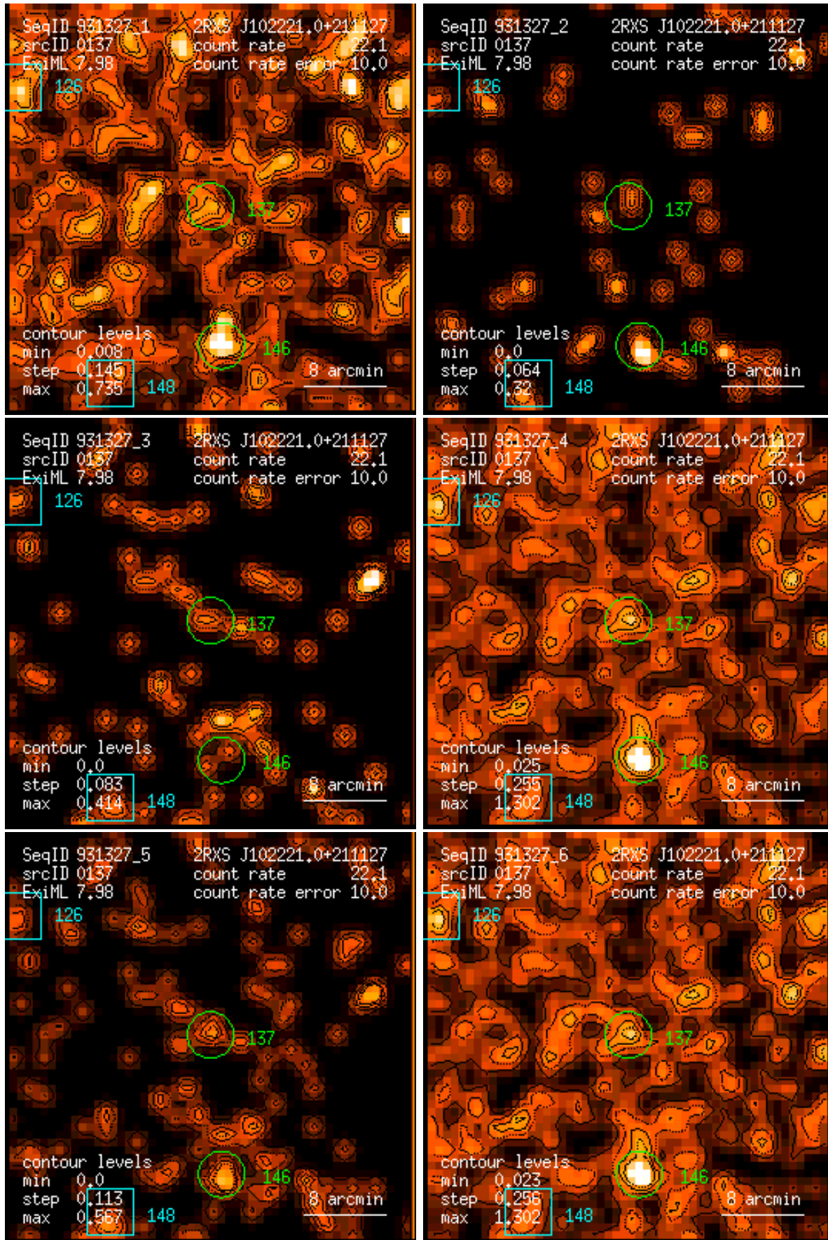
Figure 137: RASS 931327: detection 0137: band rate images, Gaussian filter: (1) PSPC channels 11 – 41, (2) 52 – 90, (3) 91 – 201, (4) 11 – 235, (5) 52 – 201, (6) 11 – 201. Broad band rates in counts/ks. Band rate contour levels in counts/ks/arcmin 2 .
