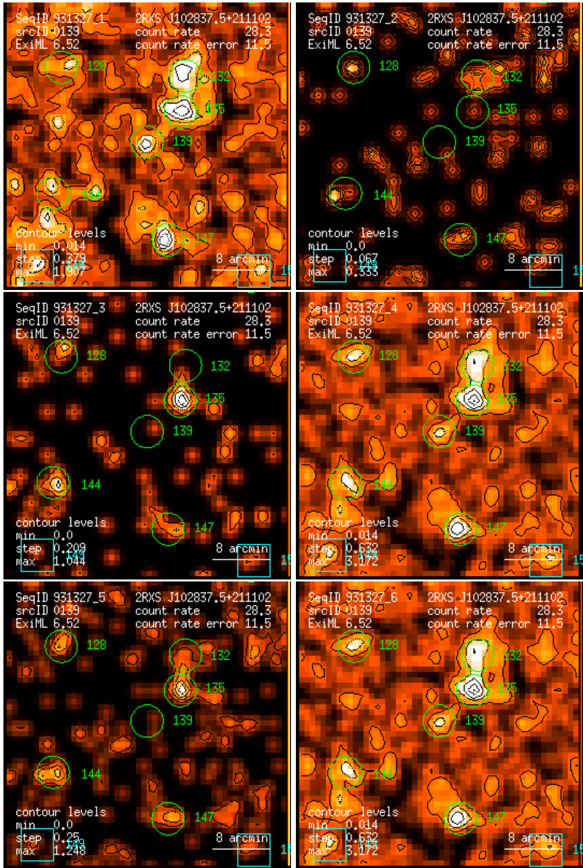
Figure 139: RASS 931327: detection 0139: band rate images, Gaussian filter: (1) PSPC channels 11 – 41, (2) 52 – 90, (3) 91 – 201, (4) 11 – 235, (5) 52 – 201, (6) 11 – 201. Broad band rates in counts/ks. Band rate contour levels in counts/ks/arcmin 2 .
