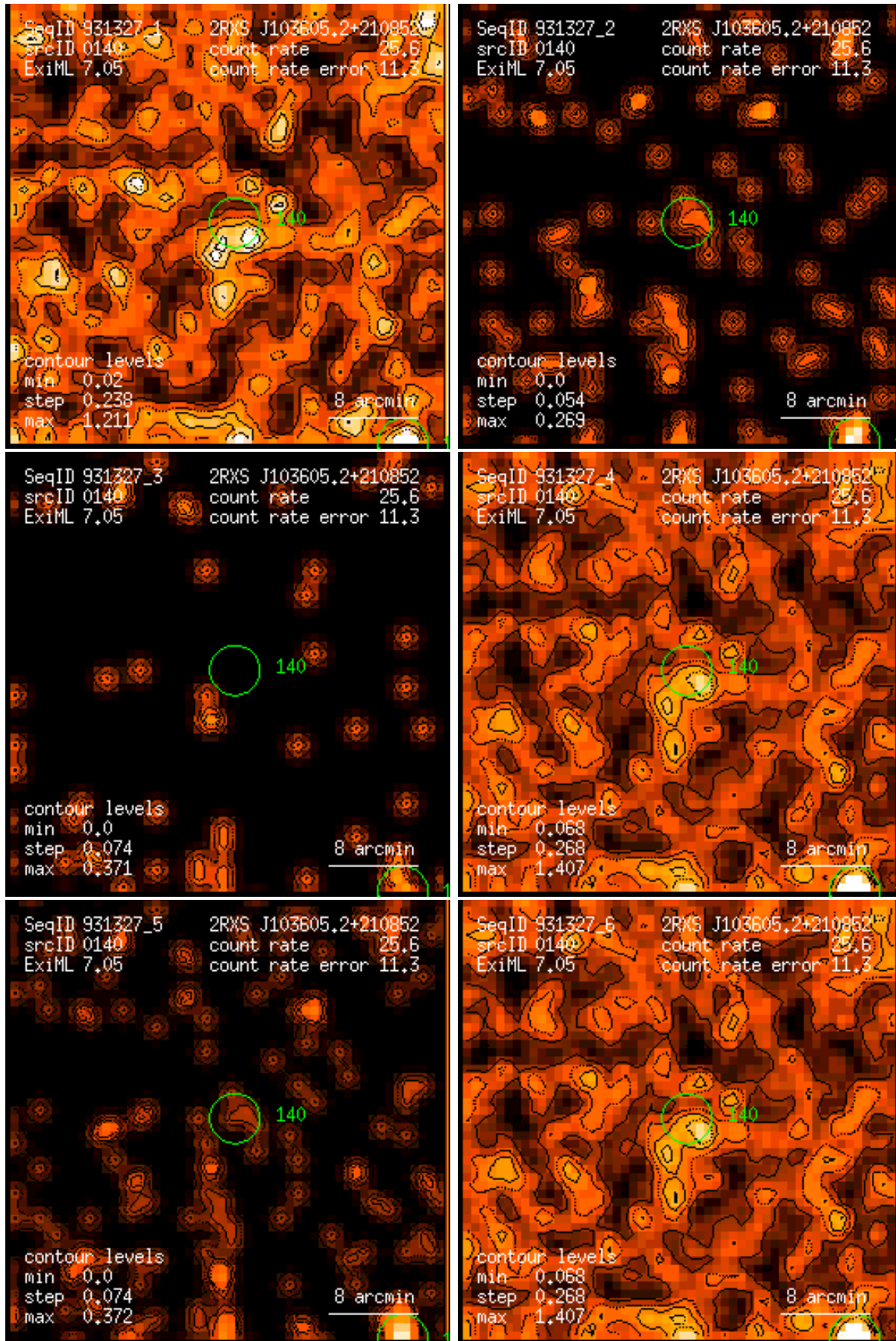
Figure 140: RASS 931327: detection 0140: band rate images, Gaussian filter: (1) PSPC channels 11 – 41, (2) 52 – 90, (3) 91 – 201, (4) 11 – 235, (5) 52 – 201, (6) 11 – 201. Broad band rates in counts/ks. Band rate contour levels in counts/ks/arcmin 2 .
