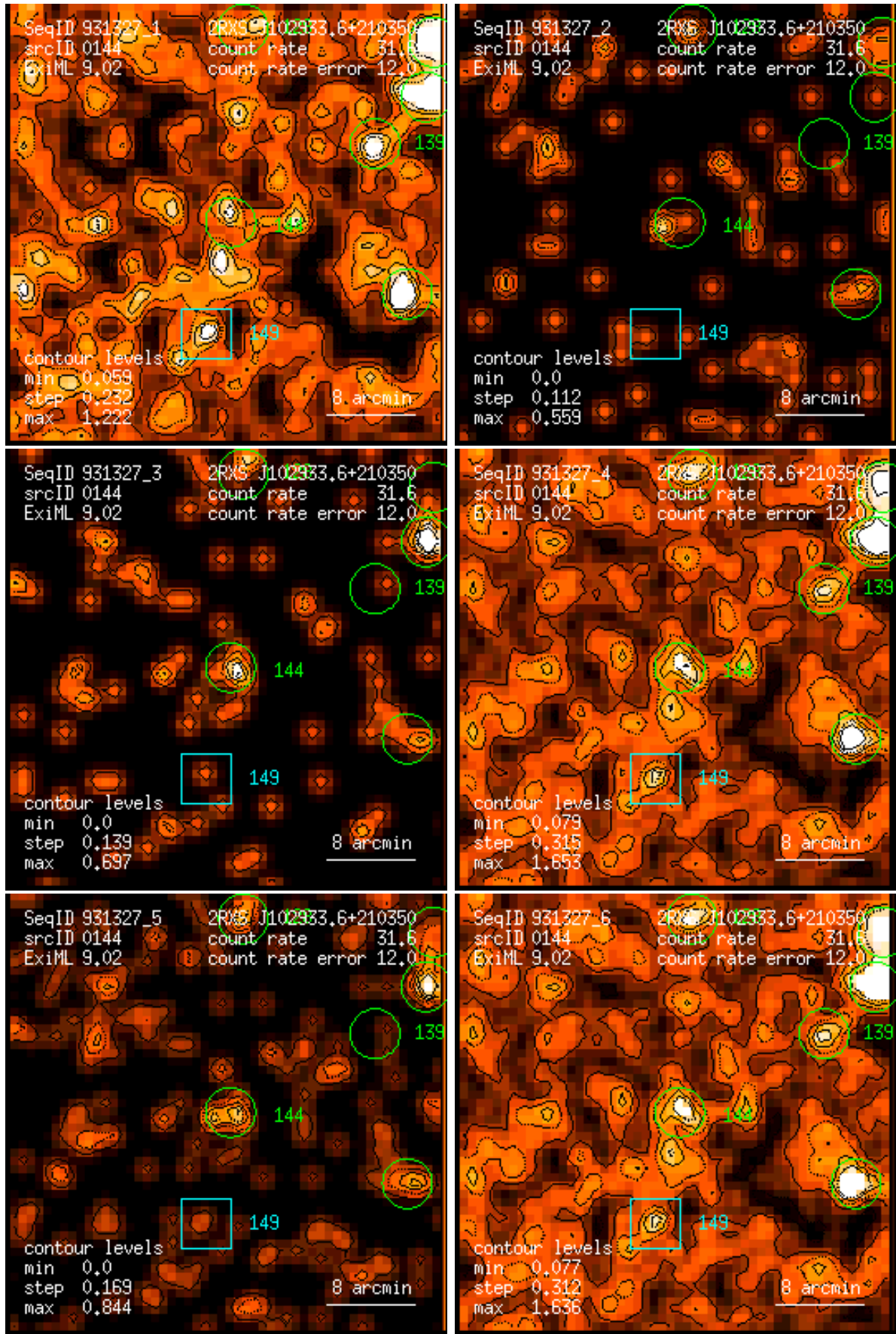
Figure 144: RASS 931327: detection 0144: band rate images, Gaussian filter: (1) PSPC channels 11 – 41, (2) 52 – 90, (3) 91 – 201, (4) 11 – 235, (5) 52 – 201, (6) 11 – 201. Broad band rates in counts/ks. Band rate contour levels in counts/ks/arcmin 2 .
