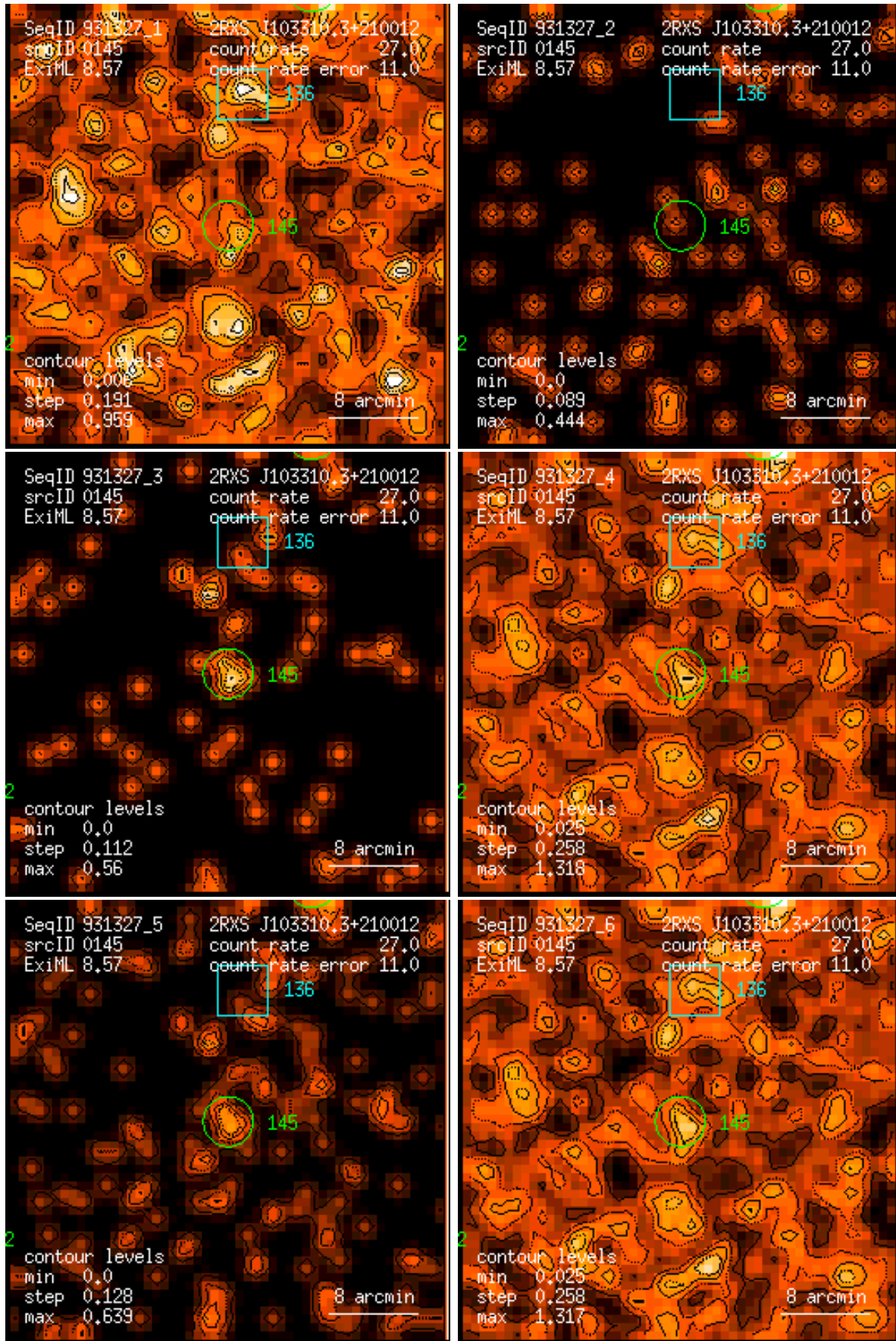
Figure 145: RASS 931327: detection 0145: band rate images, Gaussian filter: (1) PSPC channels 11 – 41, (2) 52 – 90, (3) 91 – 201, (4) 11 – 235, (5) 52 – 201, (6) 11 – 201. Broad band rates in counts/ks. Band rate contour levels in counts/ks/arcmin 2 .
